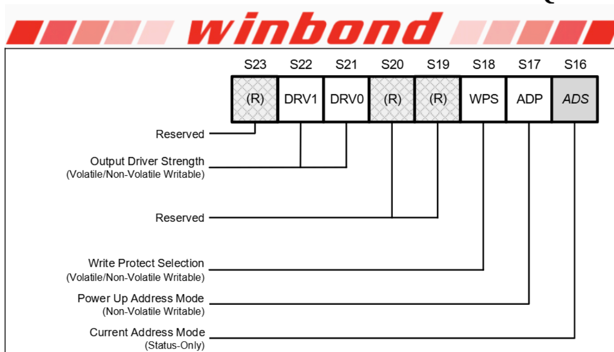
Figure 4c. Status Register-3
