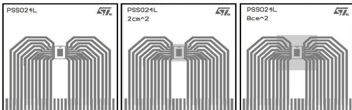
Figure 26. PowerSSO-24 PCB
