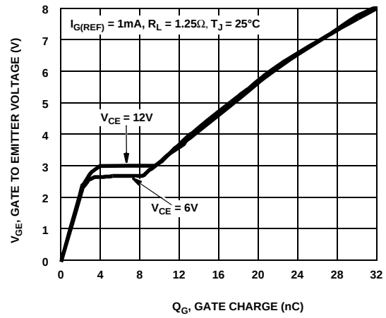
Figure 14. Gate Charge
