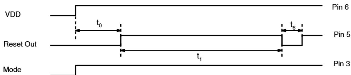
Figure 4. Power-on Reset and Switch-over Mode
