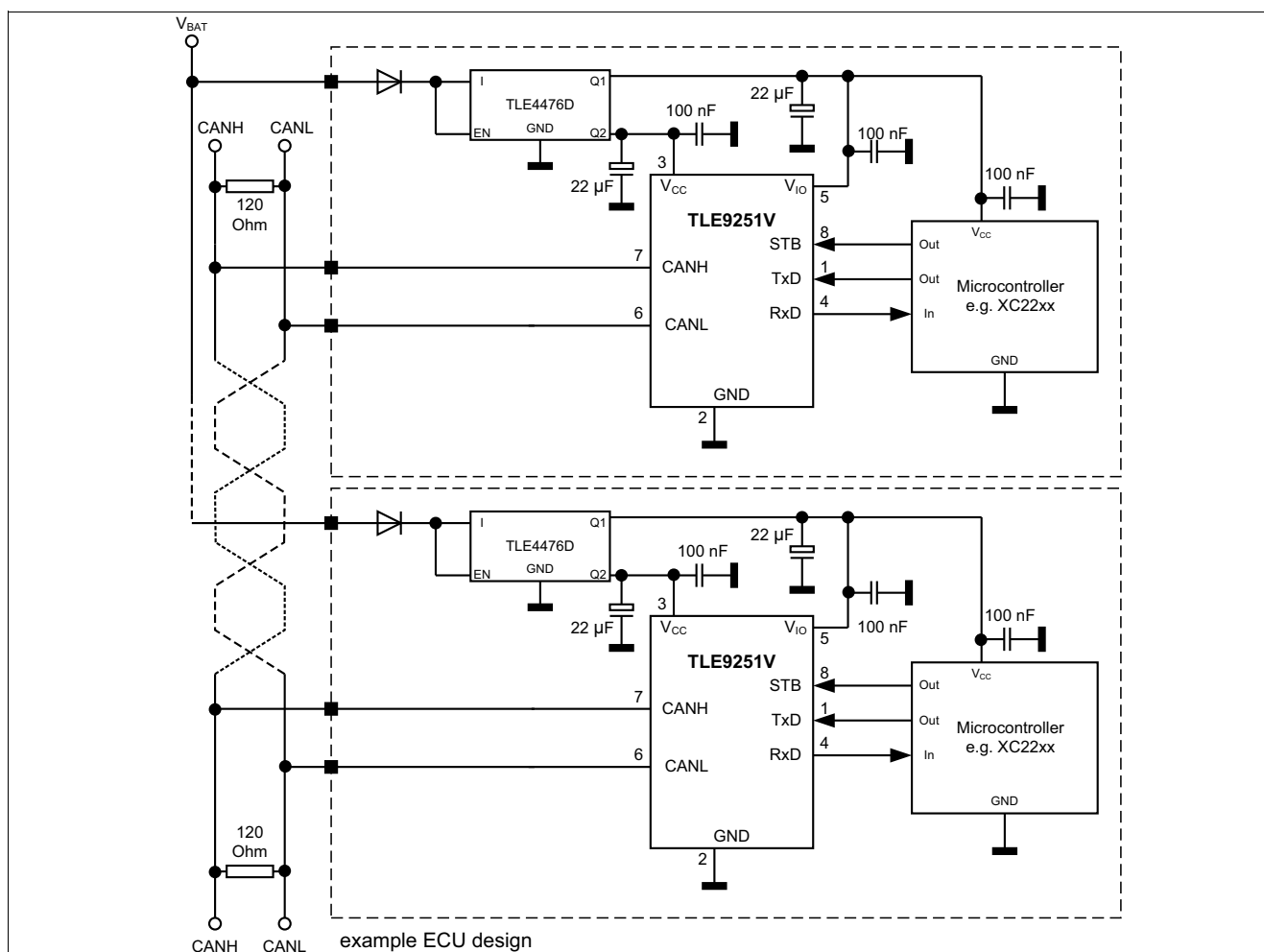
Figure 18 Application circuit
