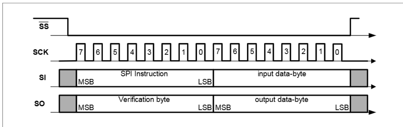
Figure 16 SPI Communication
