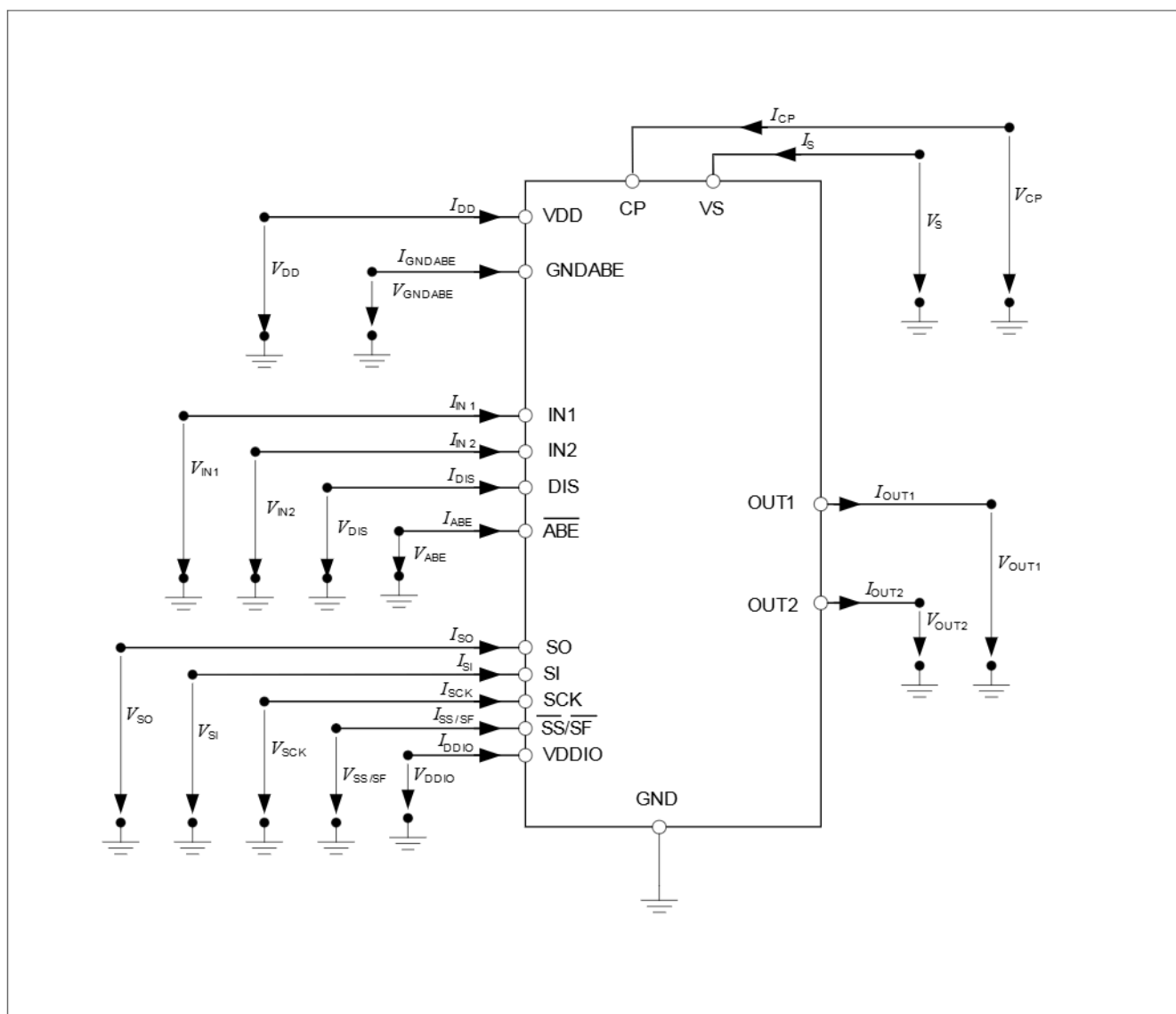
Figure 3 Terms TLE8209-2
