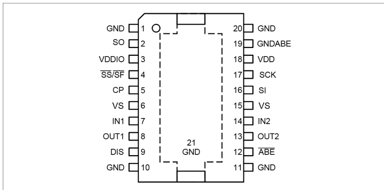
Figure 1 Pinout TLE8209-2SA
