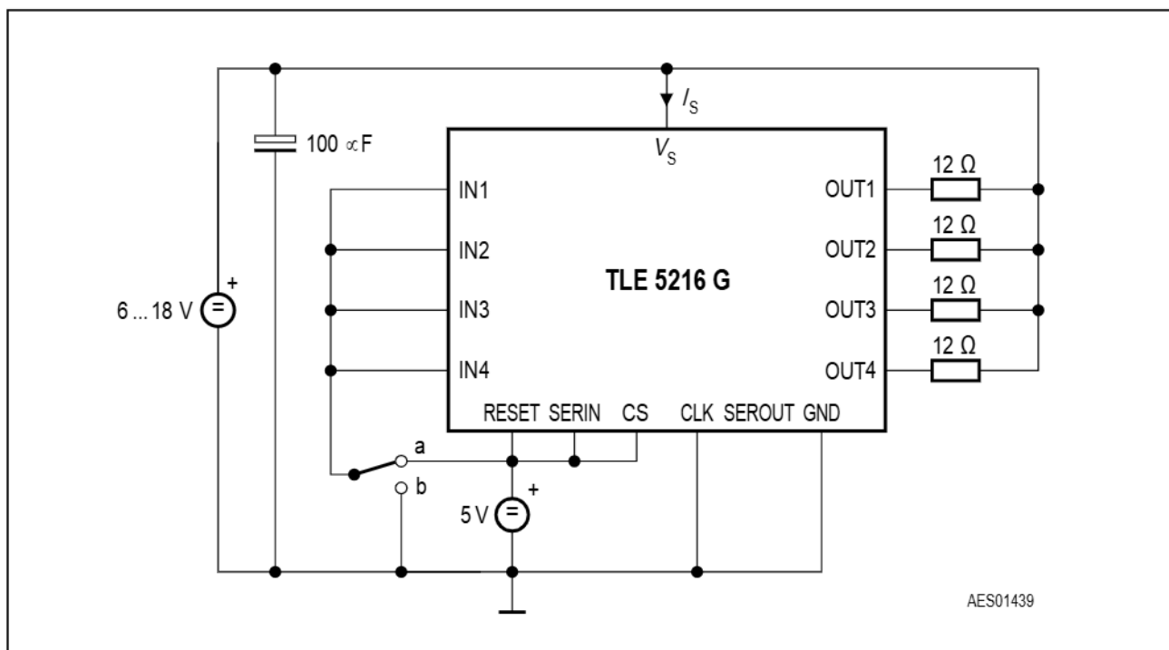
Figure 5 Test Circuit 3
