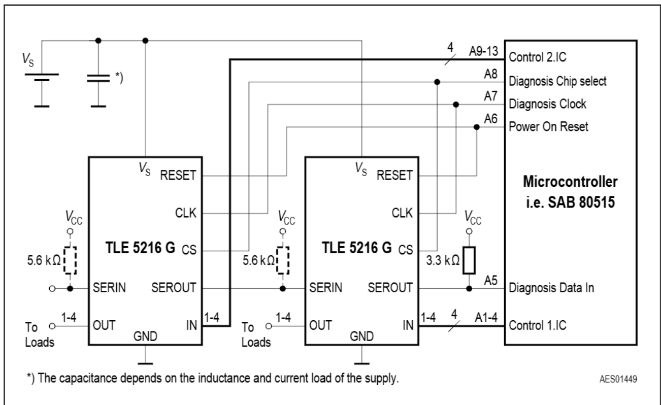
Figure 9 Application Circuit
