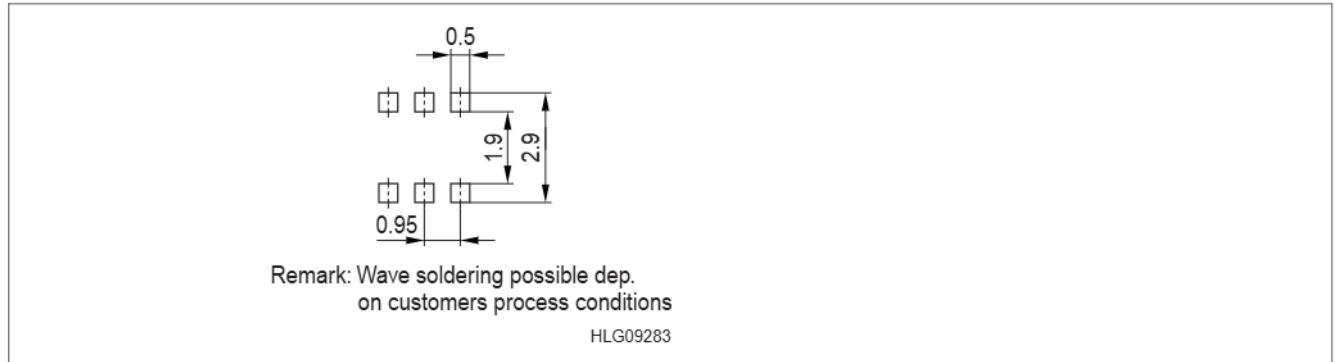
Figure 10 Footprint PG-TSOP-6-6-5
