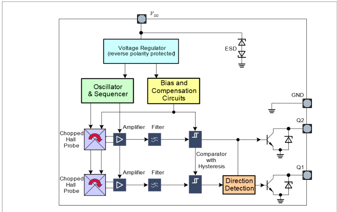
Figure 2 Block Diagram
