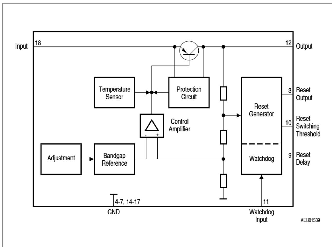
Figure 3 Block Diagram TLE 4268 G (PG-DSO-20-35)
