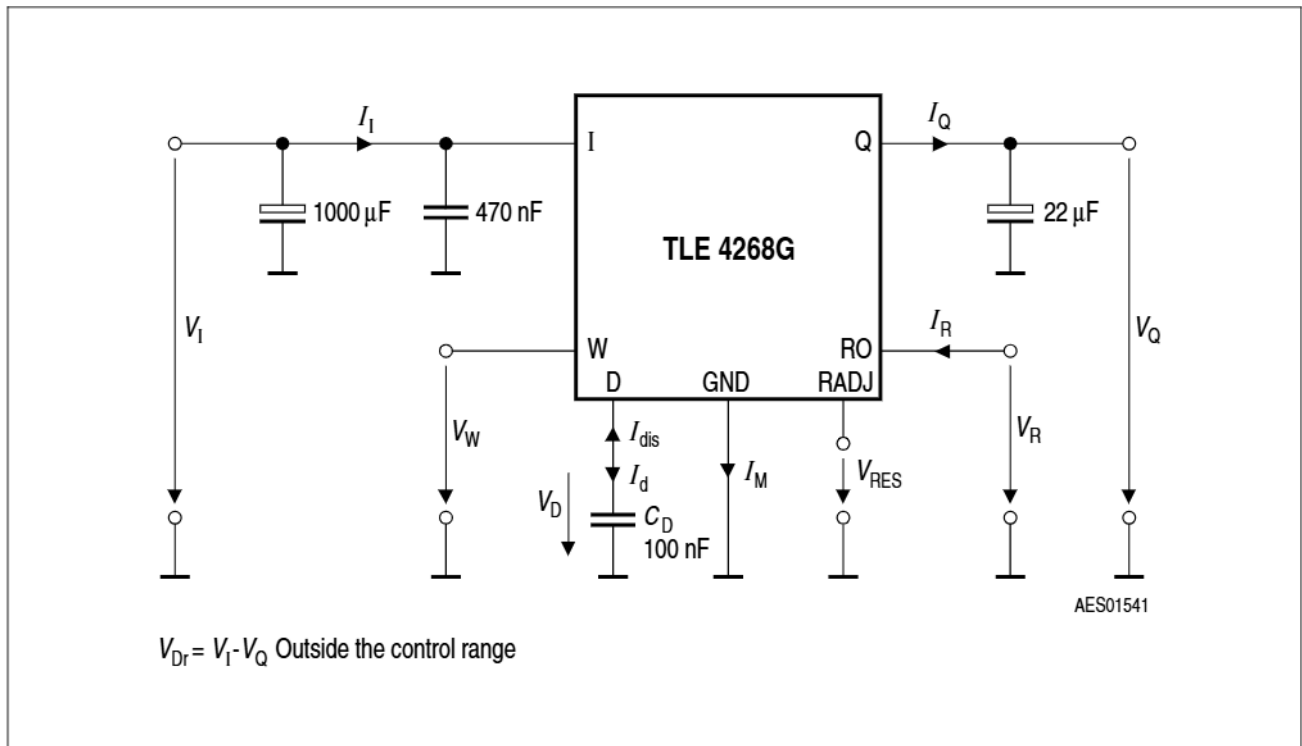
Figure 4 Test Circuit
