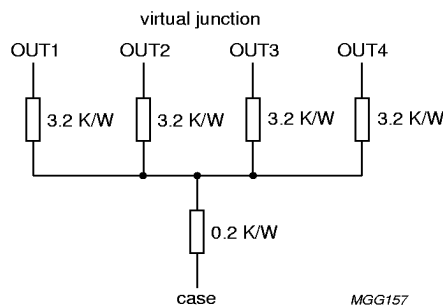
Fig.6 Equivalent thermal resistance network.
