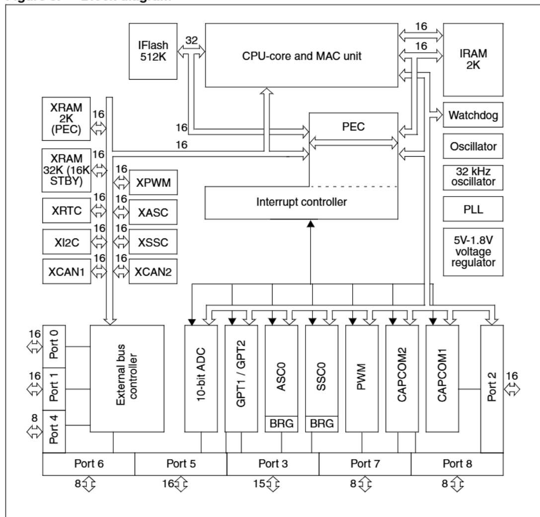
Figure 3. Block diagram
