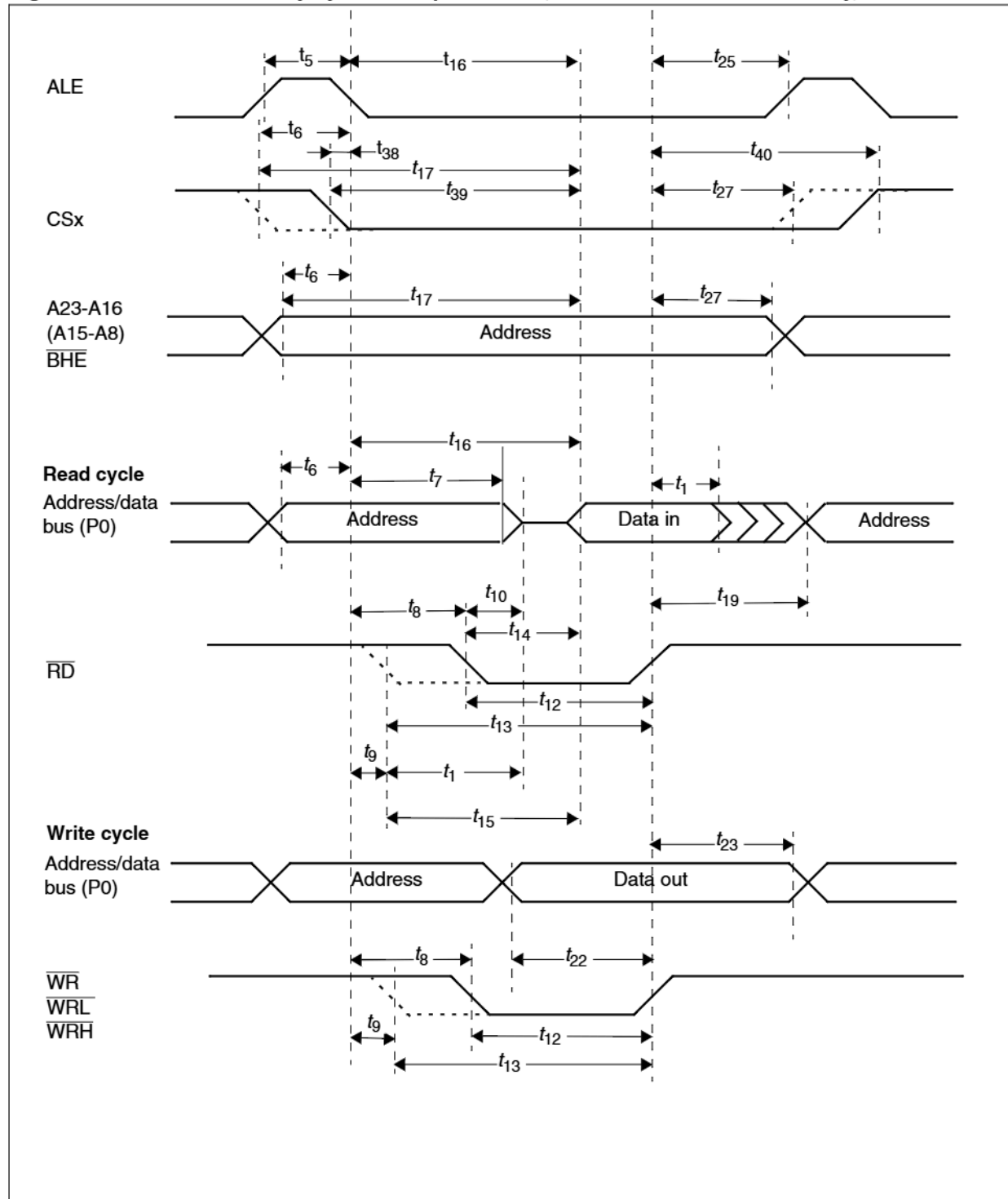
Figure 48. External memory cycle: Multiplexed bus, with/without read/write delay, normal ALE
