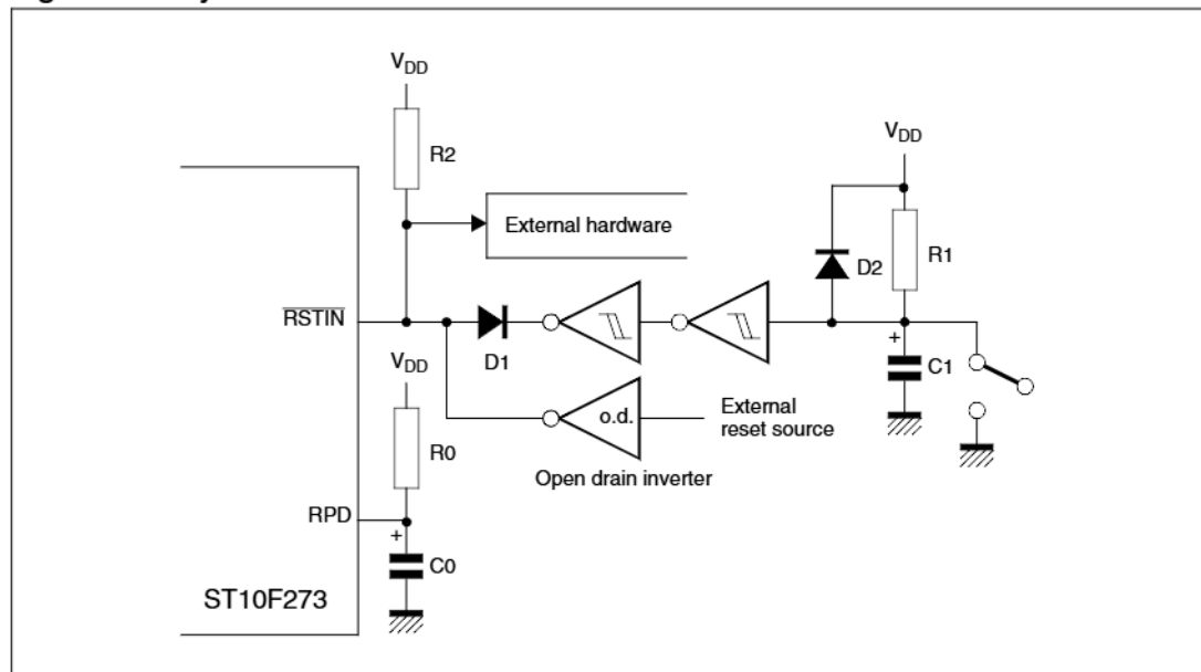
Figure 30. Internal (simplified) reset circuitry
