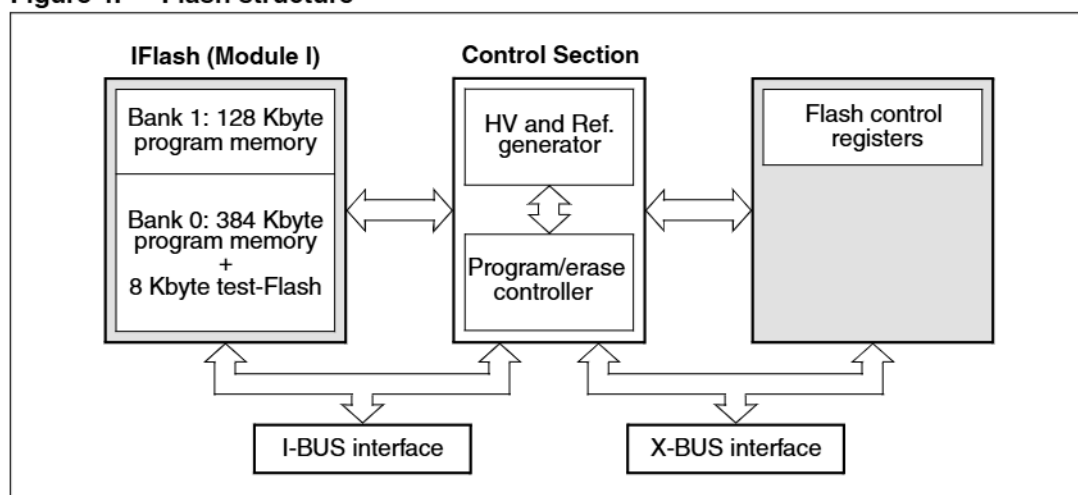
Figure 4. Flash structure
