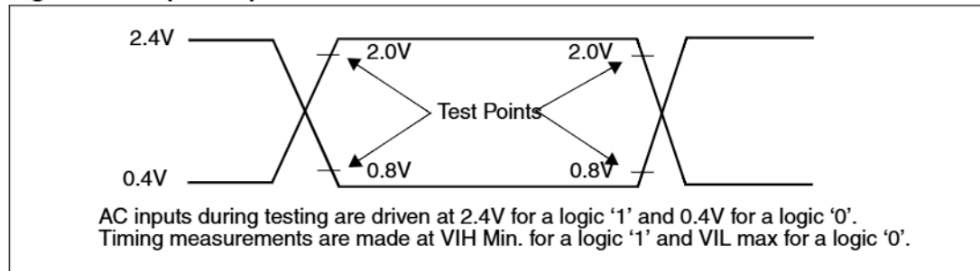
Figure 41. Input/output waveforms
