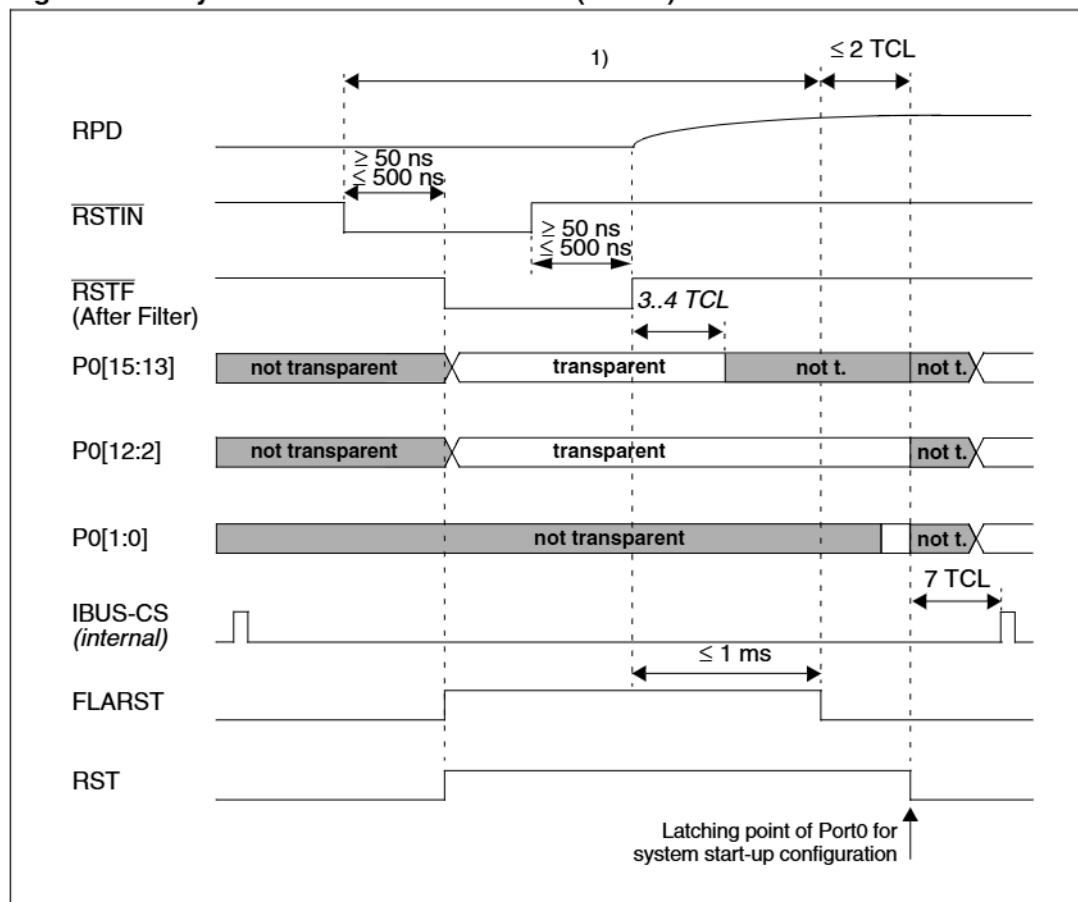
Figure 17. Asynchronous hardware RESET ( \overline{EA} = 1 )
