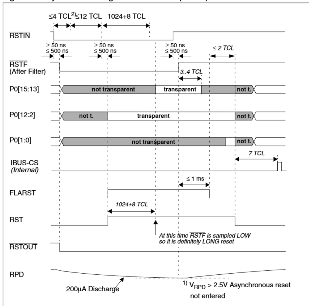
Figure 21. Synchronous long hardware RESET ( \overline{\text{EA}} = 1 )
