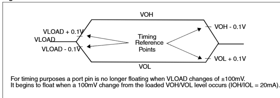
Figure 42. Float waveform
