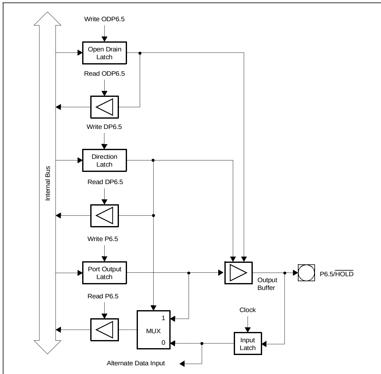
Figure 38 : Block Diagram of Pin P6.5 ( \overline{\text{HOLD}} )
