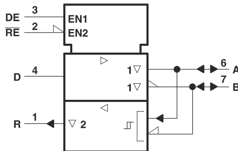
Logic Symbol 1
