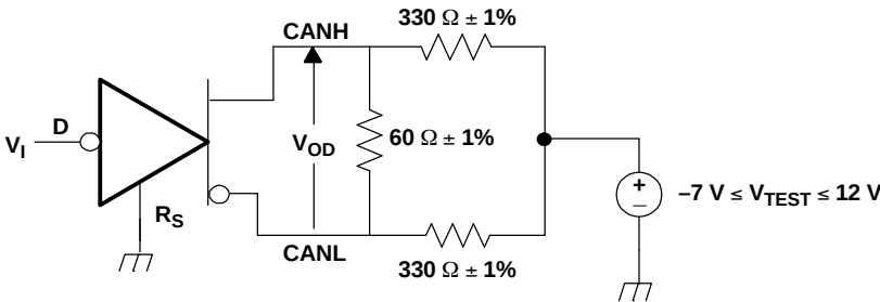
Figure 3. Driver V_{OD}
