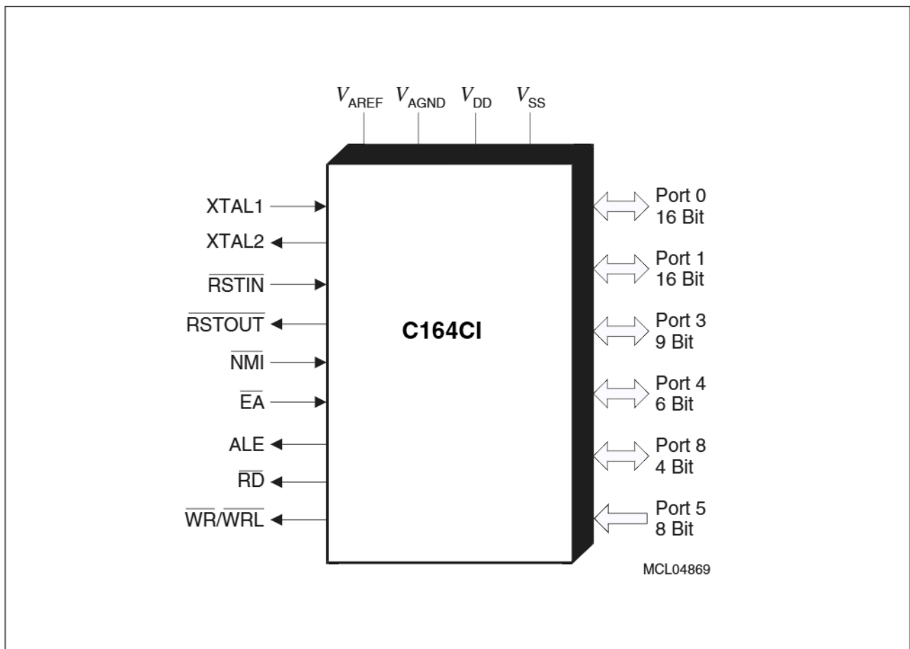
Figure 1 Logic Symbol
