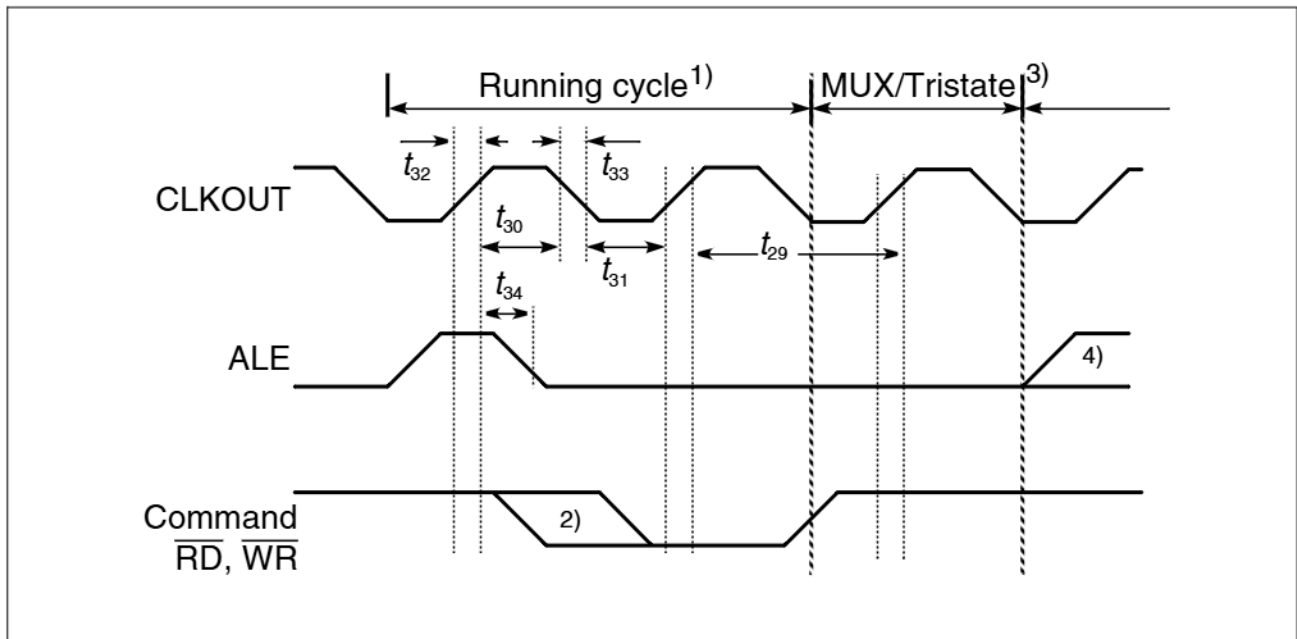
Figure 24 CLKOUT Timing
