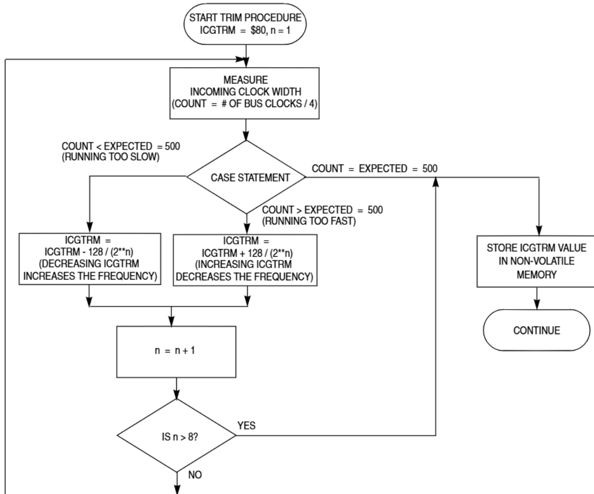
Figure 8-17. Trim Procedure
