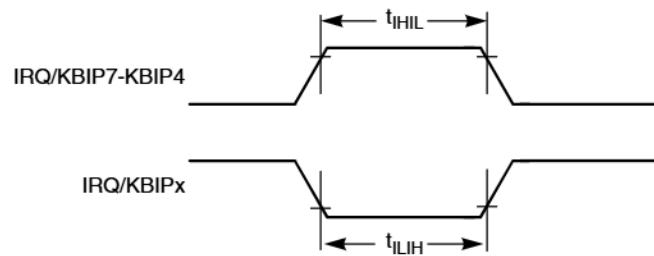
Figure A-13. IRQ/KBIPx Timing
