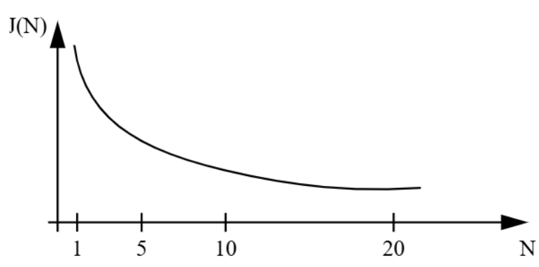
Figure A-4 Maximum bus clock jitter approximation
