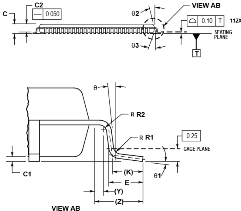
Figure C-1 112-pin LQFP mechanical dimensions (case no. 987)
