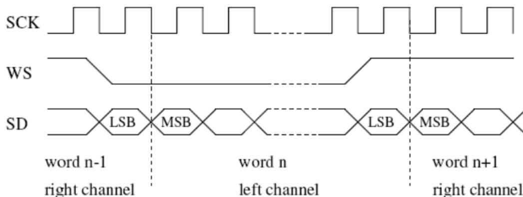
Fig. 3-14-2 I2S Transmitter
