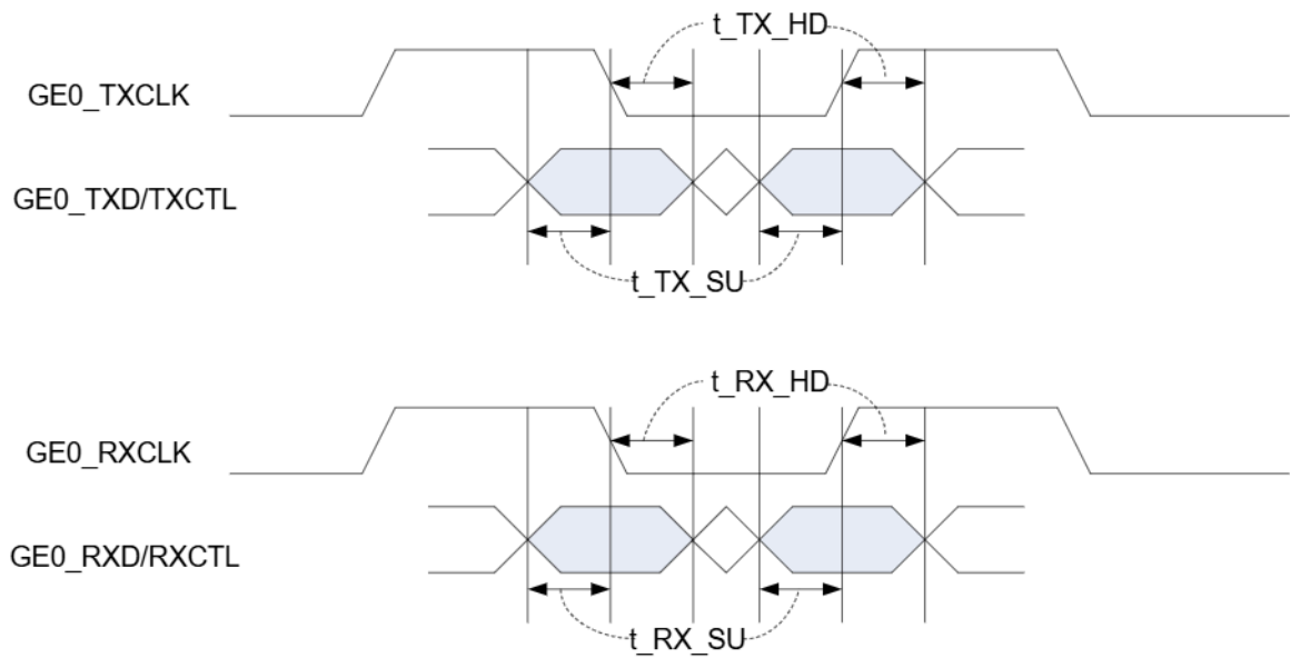
Fig. 2-6-3 RGMII Interface
