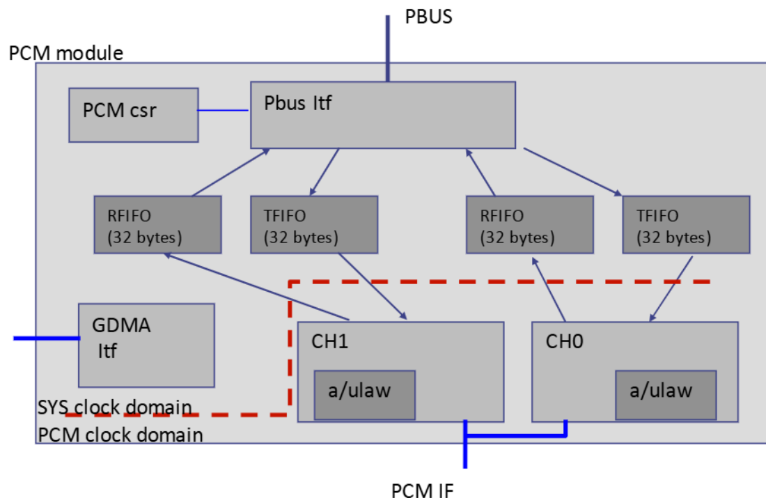
Fig. 3-13-1 PCM Controller Block Diagram
