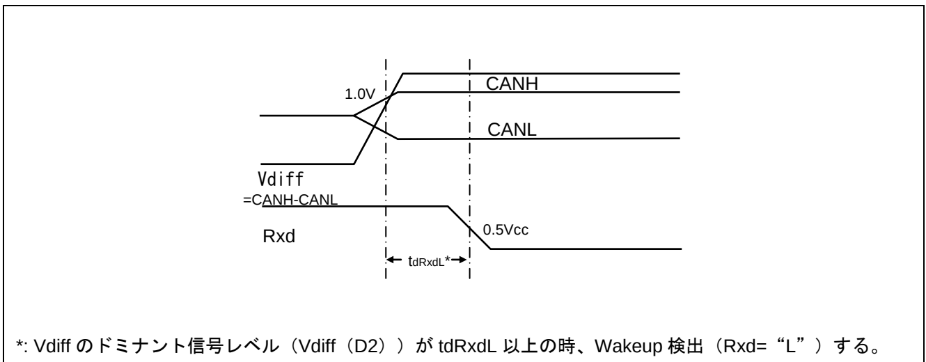
図 4 Wakeup (MODE= "H")
