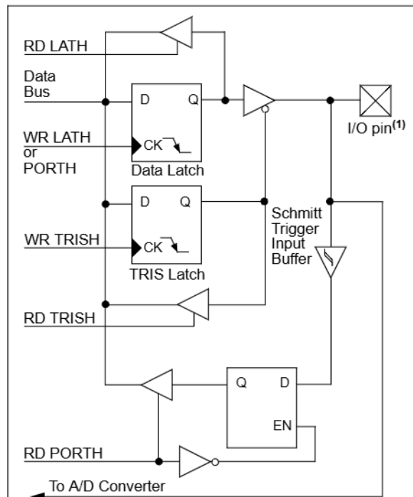
FIGURE 10-18: RH7:RH4 PINS BLOCK DIAGRAM IN I/O MODE
