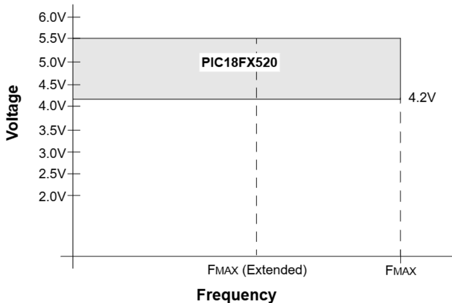
FIGURE 26-1: PIC18F6520/8520 VOLTAGE-FREQUENCY GRAPH (INDUSTRIAL, EXTENDED)
