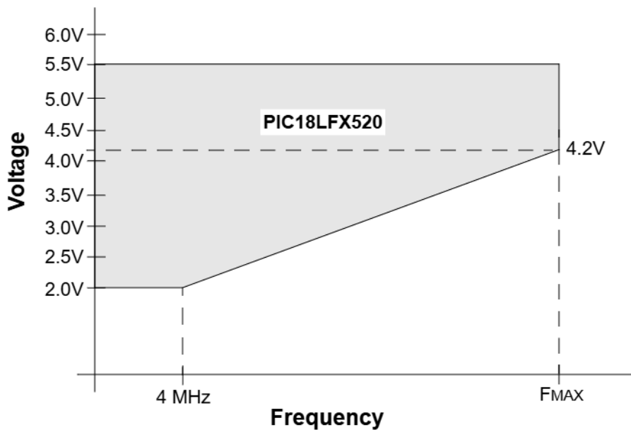
FIGURE 26-2: PIC18LF6520/8520 VOLTAGE-FREQUENCY GRAPH (INDUSTRIAL)
