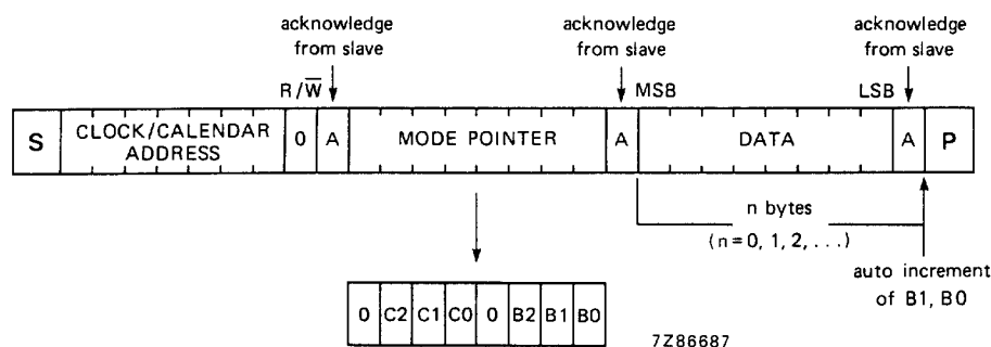
Fig.9 Master transmitter transmits to clock/calendar slave receiver.
