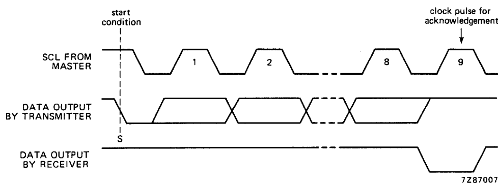
Fig.6 Acknowledge on the I 2 C-bus.
