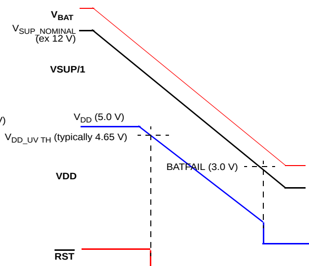
Case 2: “V DD_UV 4.6V”, with bit Crank = 1
