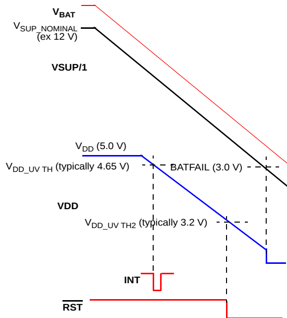
Case 2: “V DD_UV 3.2V”, with bit Crank = 1
