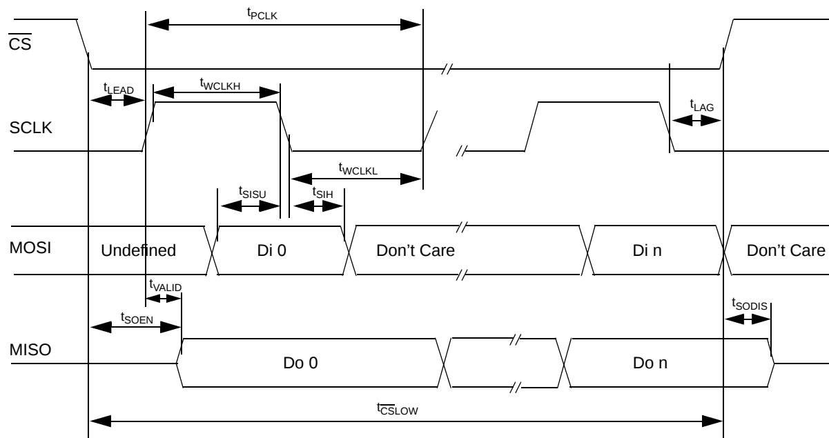
Figure 14. SPI Timings
