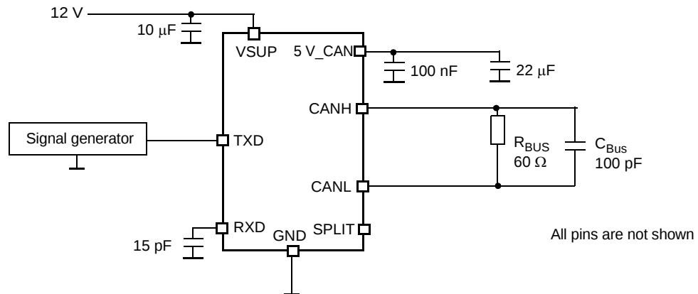
Figure 17. Test Circuit for CAN Timing Characteristics
