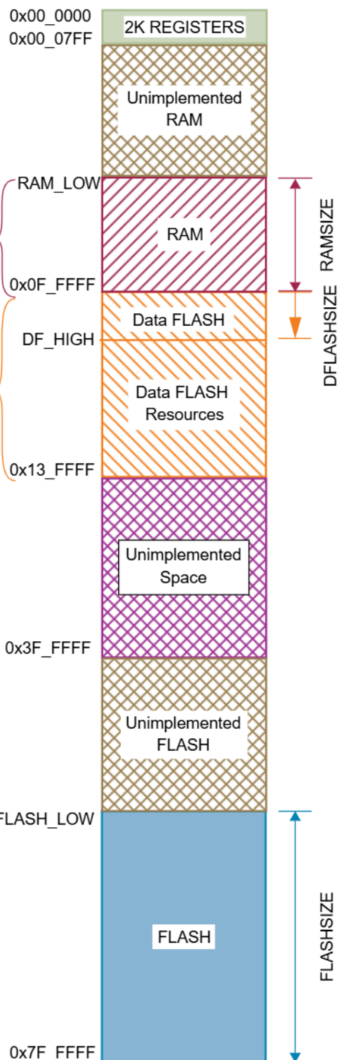
Figure 3-19. S12X CPU & BDM Global Address Mapping
