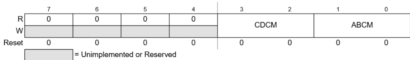
Figure 6-6. Debug Control Register2 (DBGCR2)
