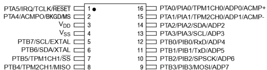
Figure 2-3. 16-Pin TSSOP
