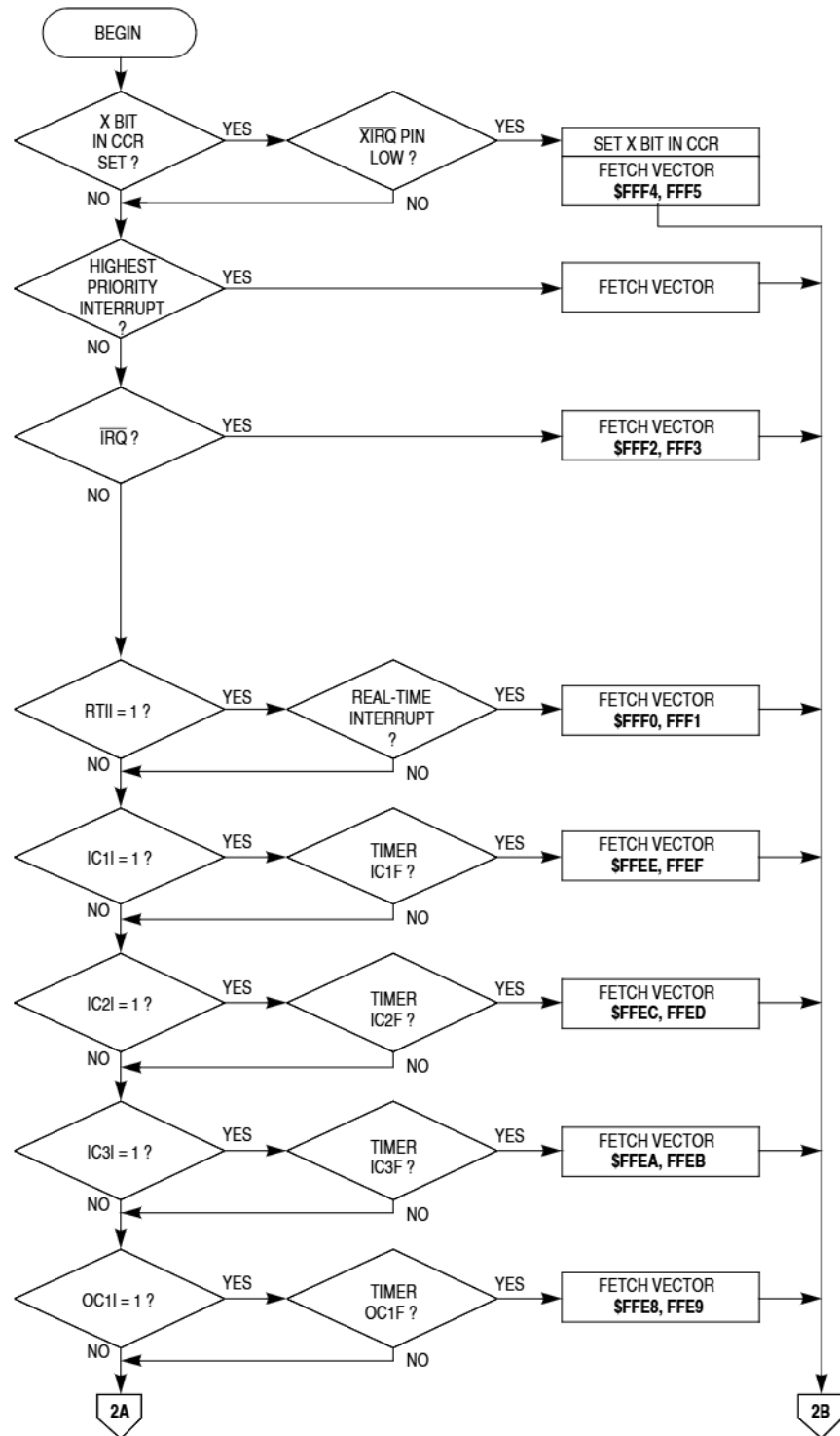
Figure 5-6. Interrupt Priority Resolution (Sheet 1 of 2)
