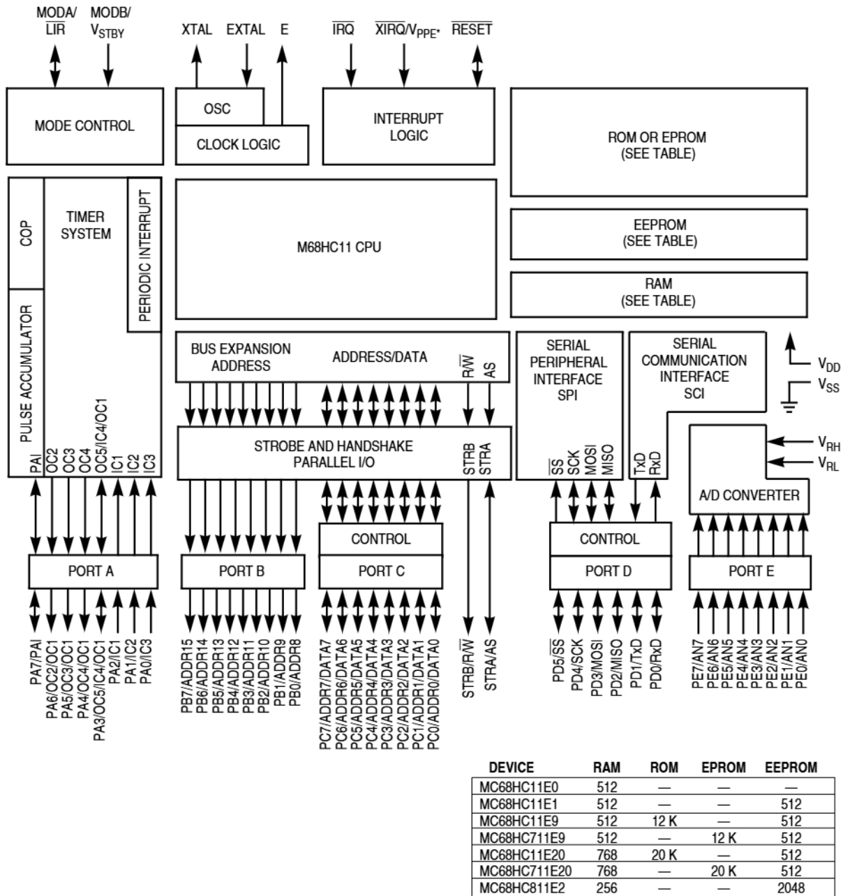
Figure 1-1. M68HC11 E-Series Block Diagram
