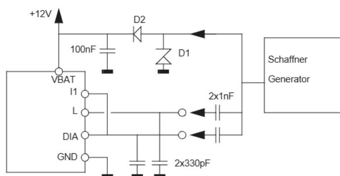
Figure 26. Test Circuit for Transient Schaffner Pulses
