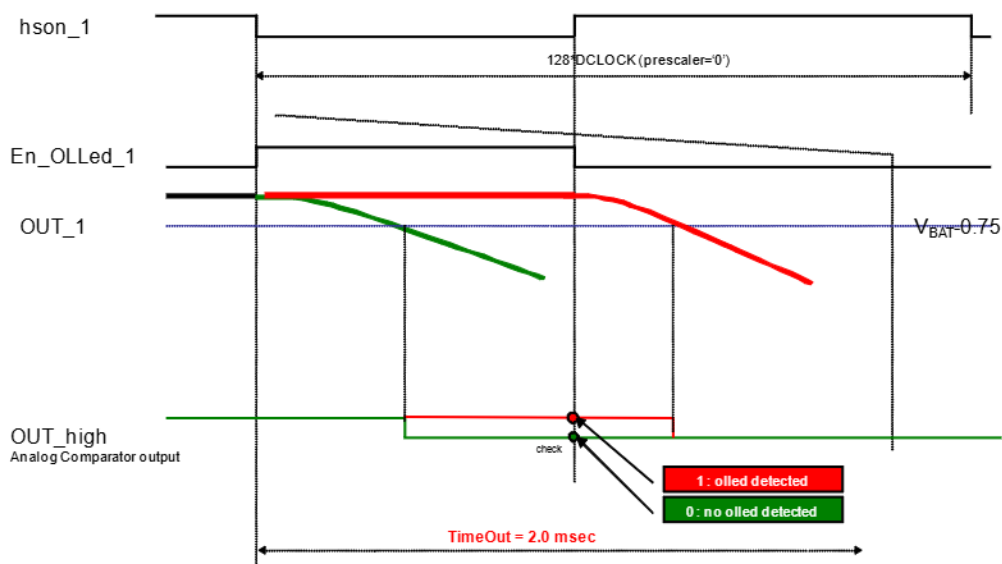
Figure 25. Open load in on state for LED in PWM operation (off time < 2.0 ms)
