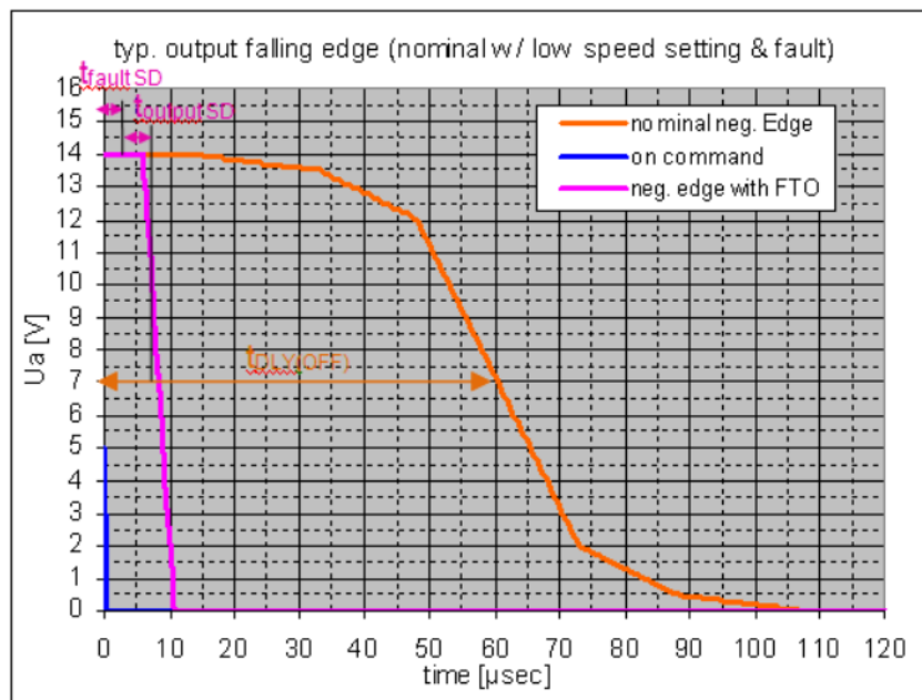
Figure 12. Power output switching in nominal operation and in case of a fault
