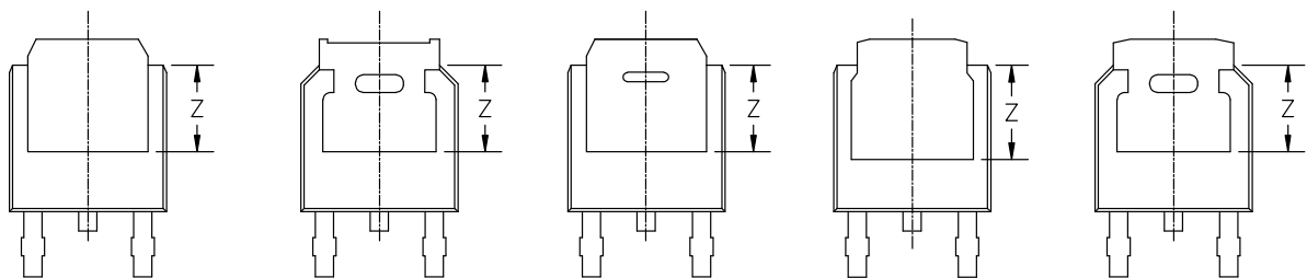
BOTTOM VIEW
