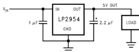
Figure 26. Typical Application Circuit
