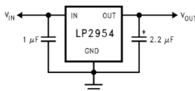
Figure 27. 5V Regulator
