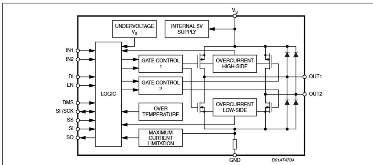
Figure 2. Block Diagram
