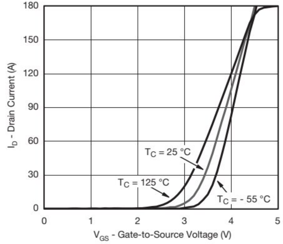
Transfer Characteristics
