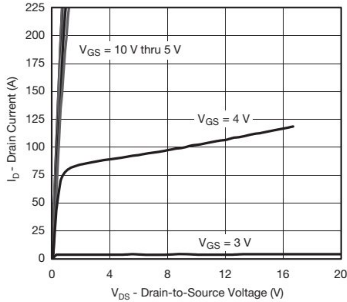
Output Characteristics
