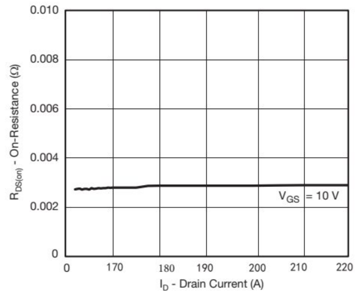
On-Resistance vs. Drain Current
