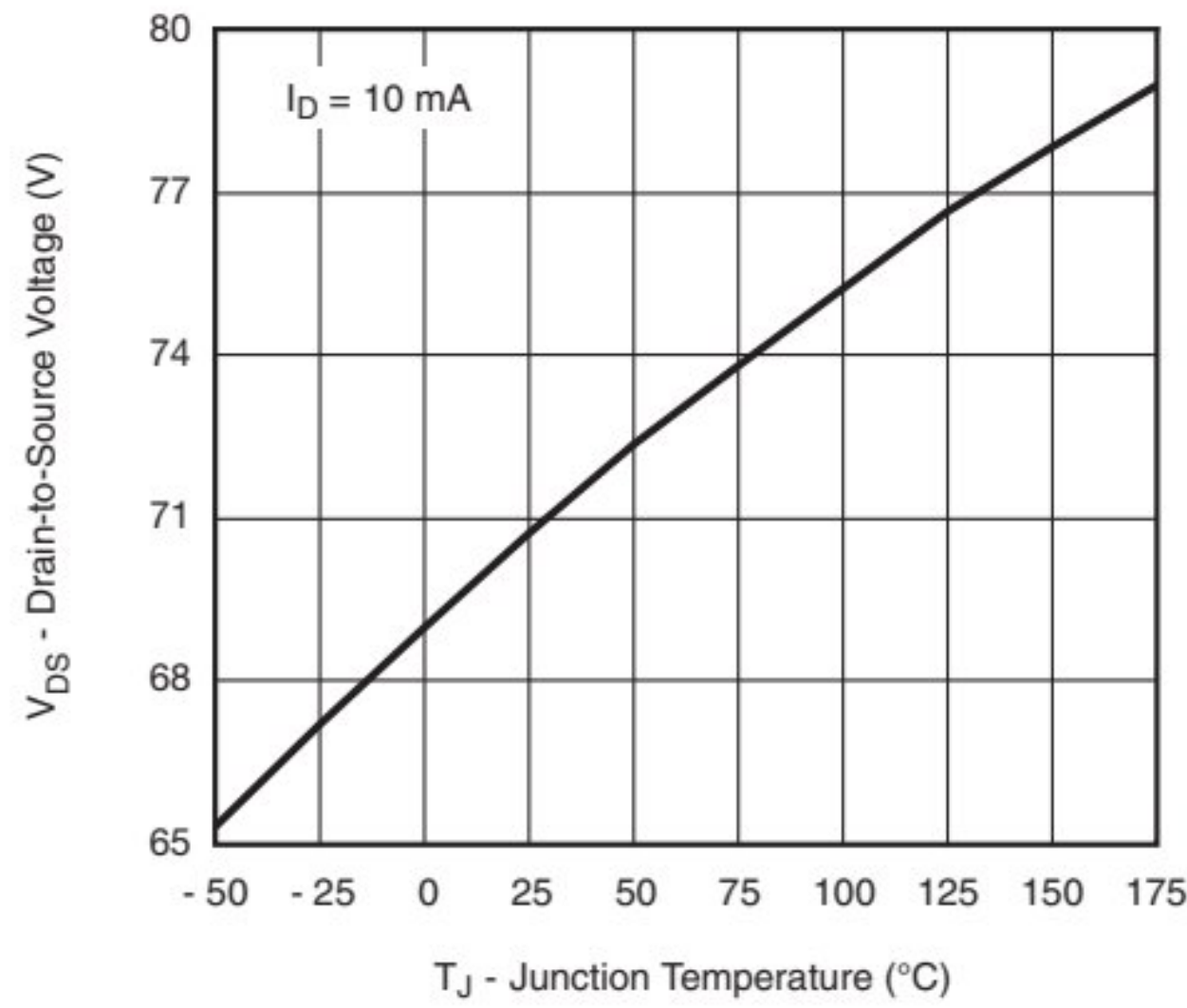
Drain Source Breakdown vs. Junction Temperature
