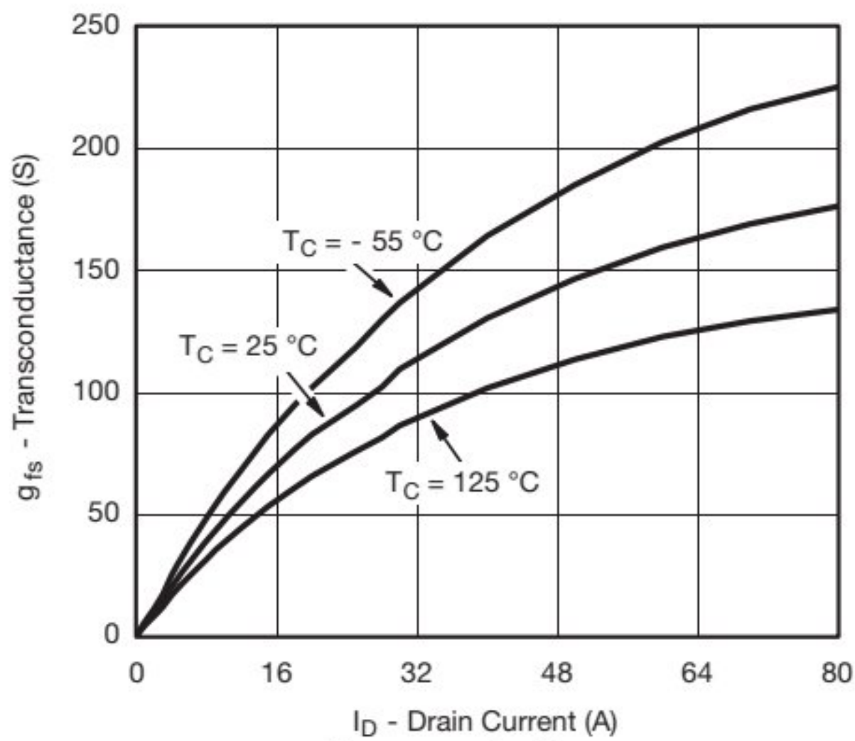
Transconductance
