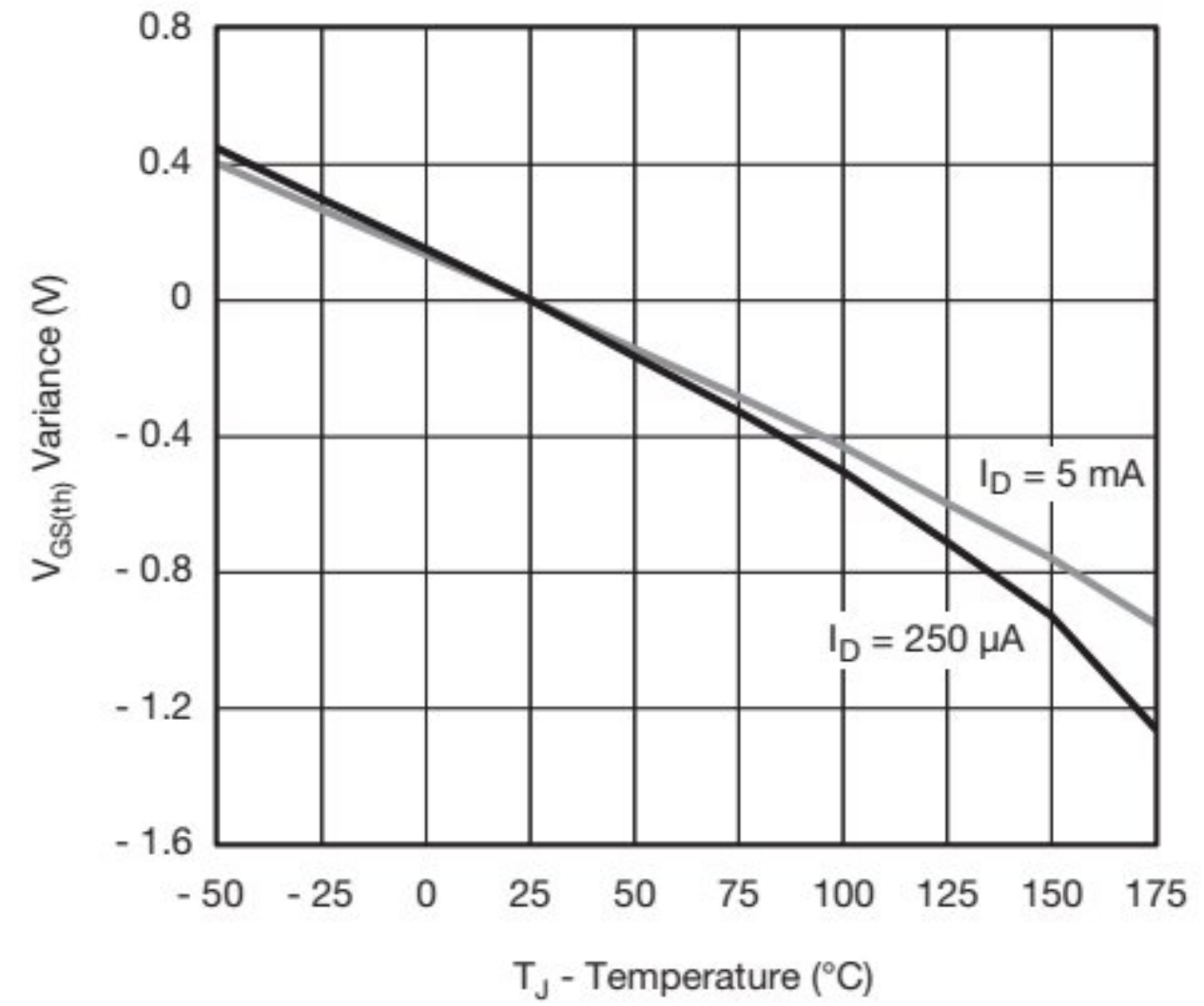
Threshold Voltage
