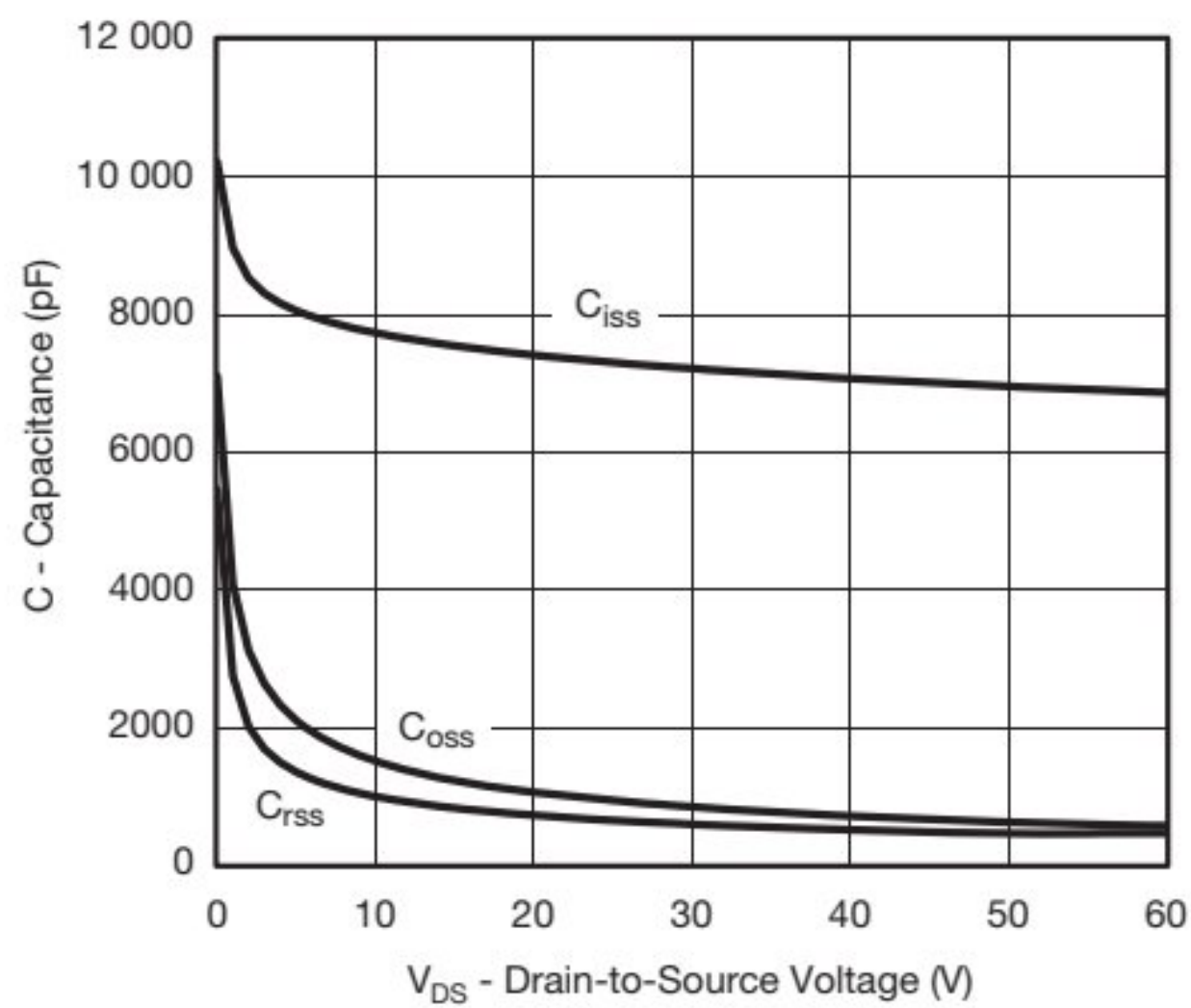
Capacitance
