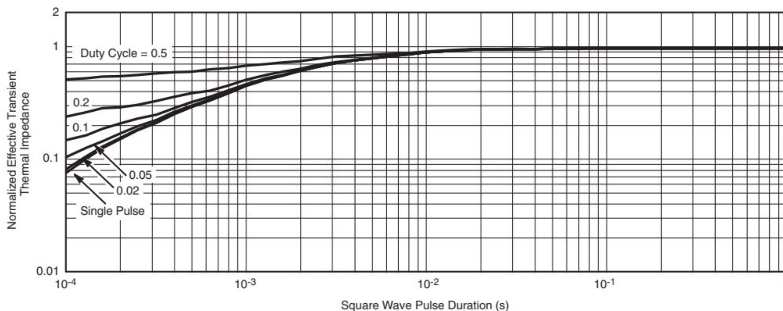
Normalized Thermal Transient Impedance, Junction-to-Case
