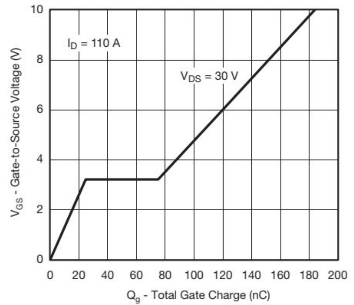
Gate Charge
