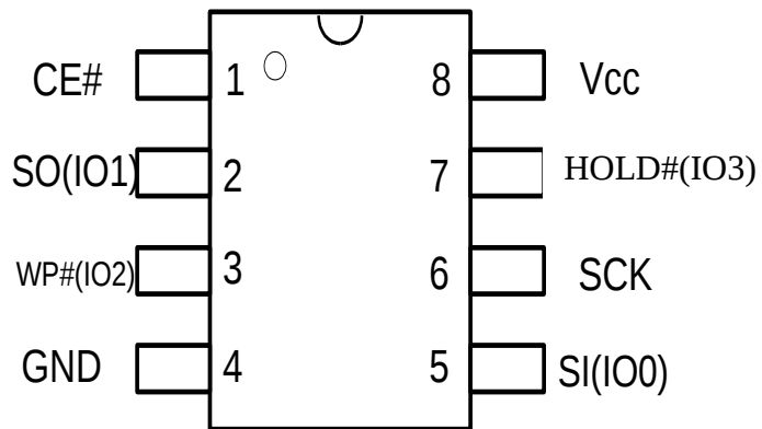
8-Pin PDIP
