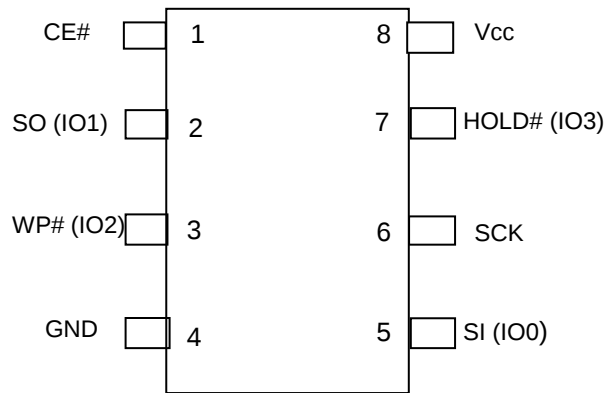
8-Pin SOIC/VVSOP
