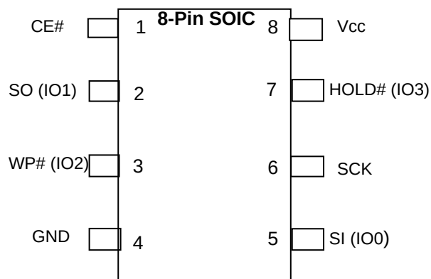
8-Pin SOIC/VSOP
