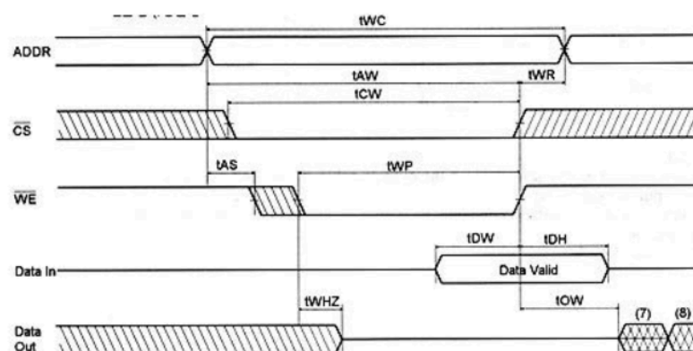
WRITE CYCLE 2 (/OE Low Fixed)
