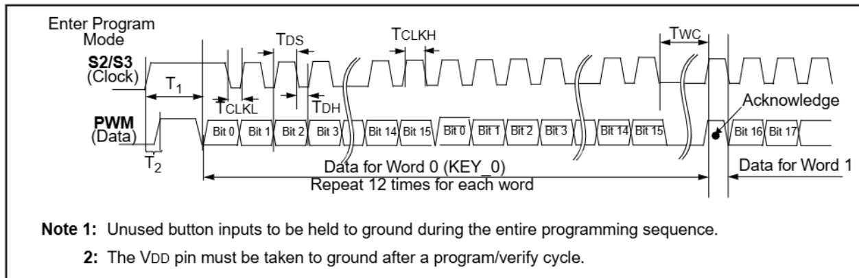
FIGURE 6-1: PROGRAMMING WAVEFORMS
