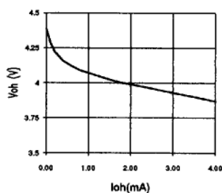
Voh vs Ioh
