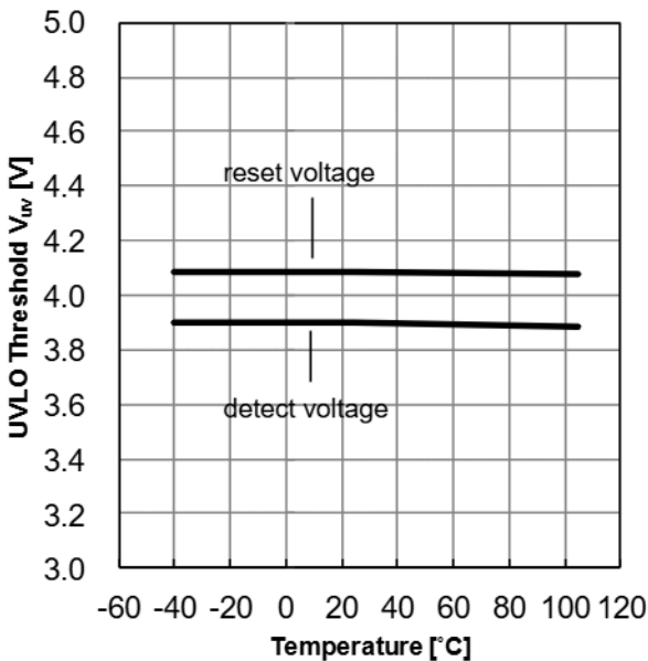
Figure 14. UVLO Threshold vs Temperature
