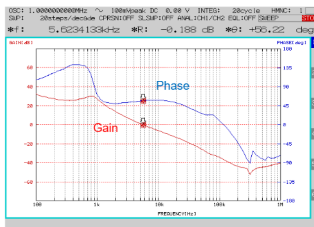
Figure 28. Frequency Characteristics (IOUT= 3.5A)
