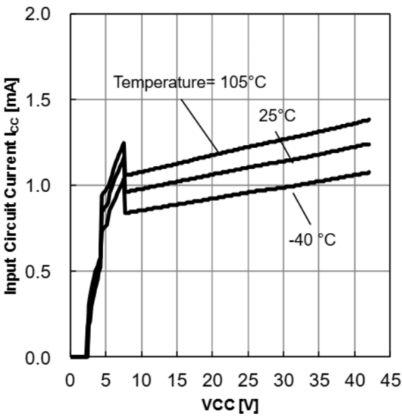
Figure 12. Input Circuit Current vs Input Voltage ( V_{FB}= 1.2V )
