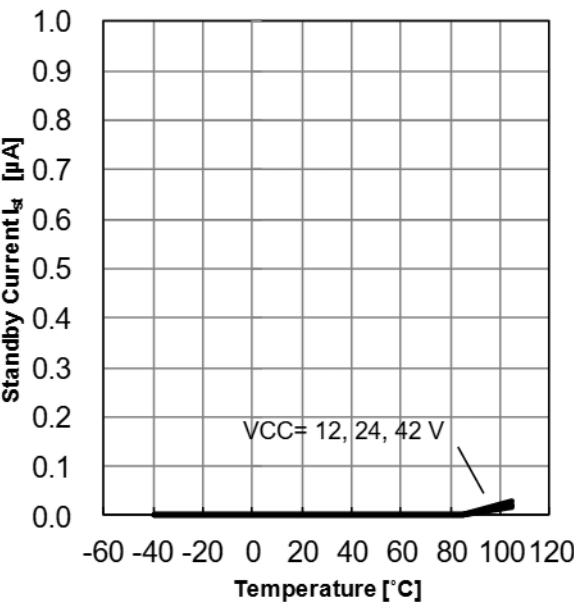
Figure 11. Standby Current vs Temperature
