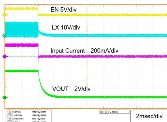
Figure 30. Shutdown Waveform (IOUT= 0.5A)
