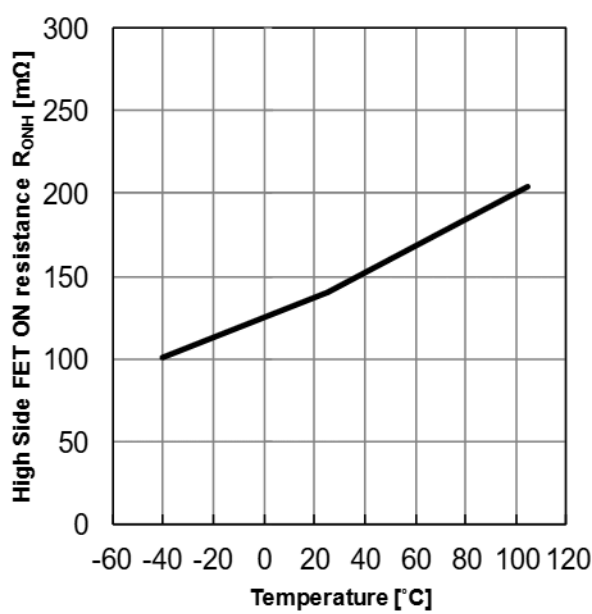
Figure 20. High Side FET R_{ON} vs Temperature
