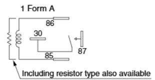
Schematic (Bottom view)
