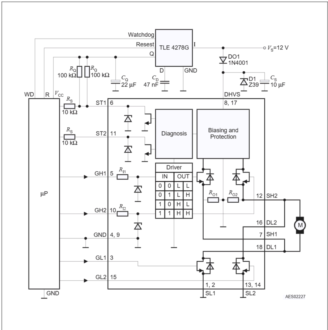
Figure 4 Application Circuit
