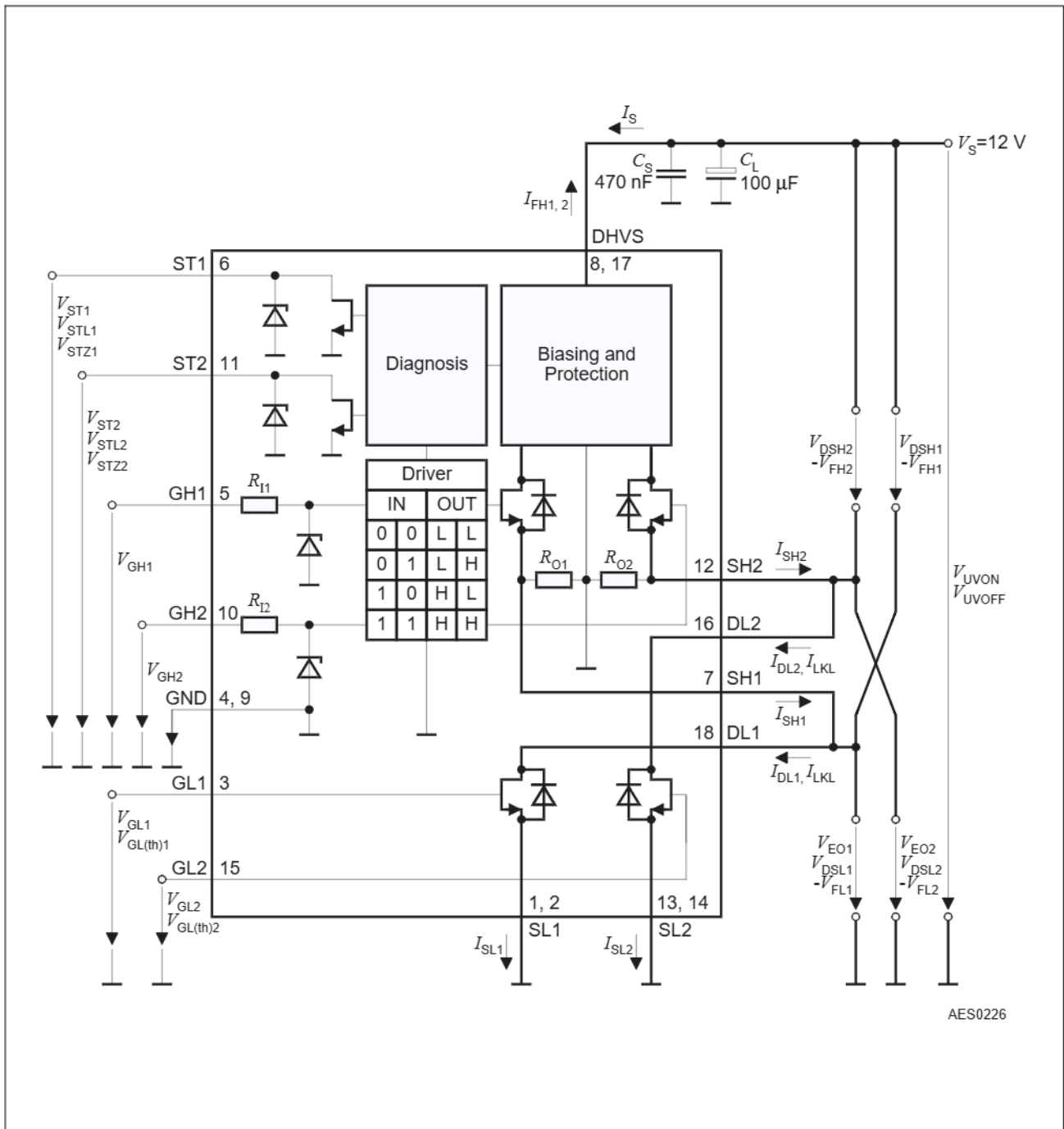
Figure 3 Test Circuit
