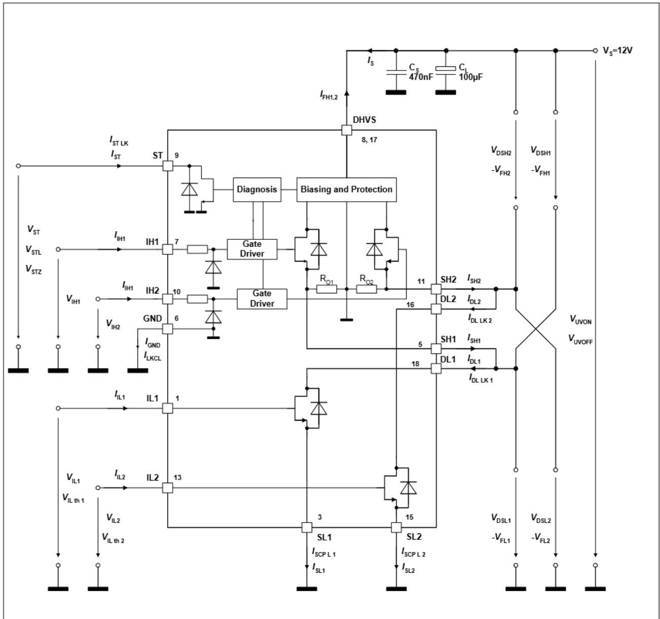
Figure 3 Test Circuit
