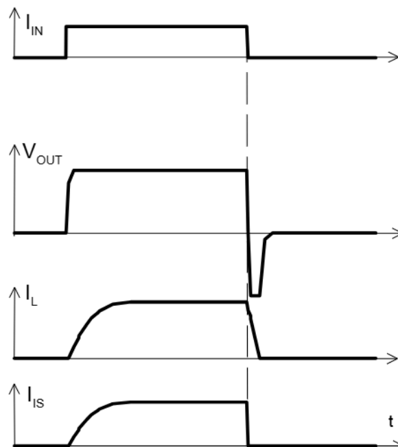
Figure 2c: Switching an inductive load:
