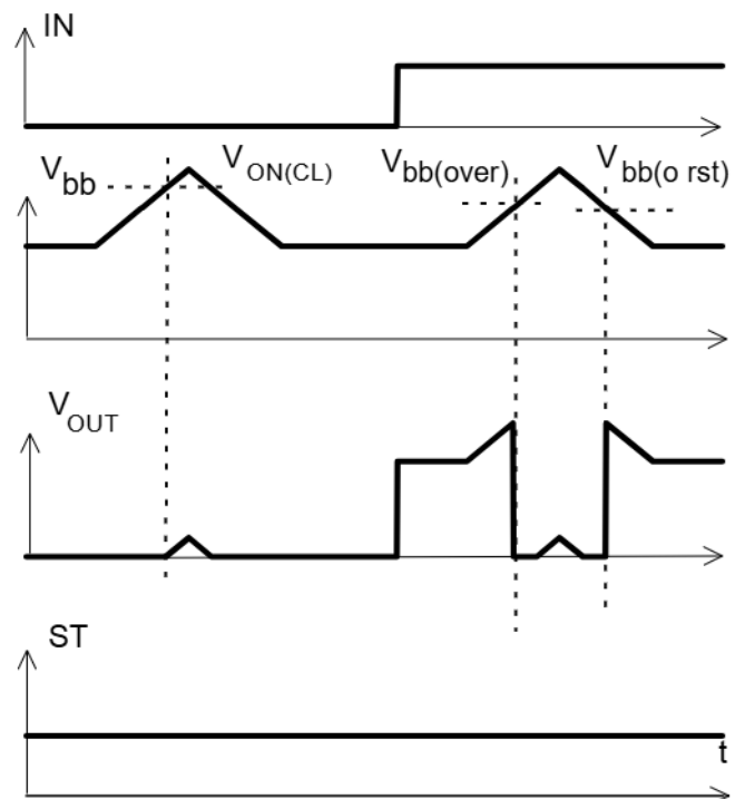
Figure 7a: Overvoltage:
