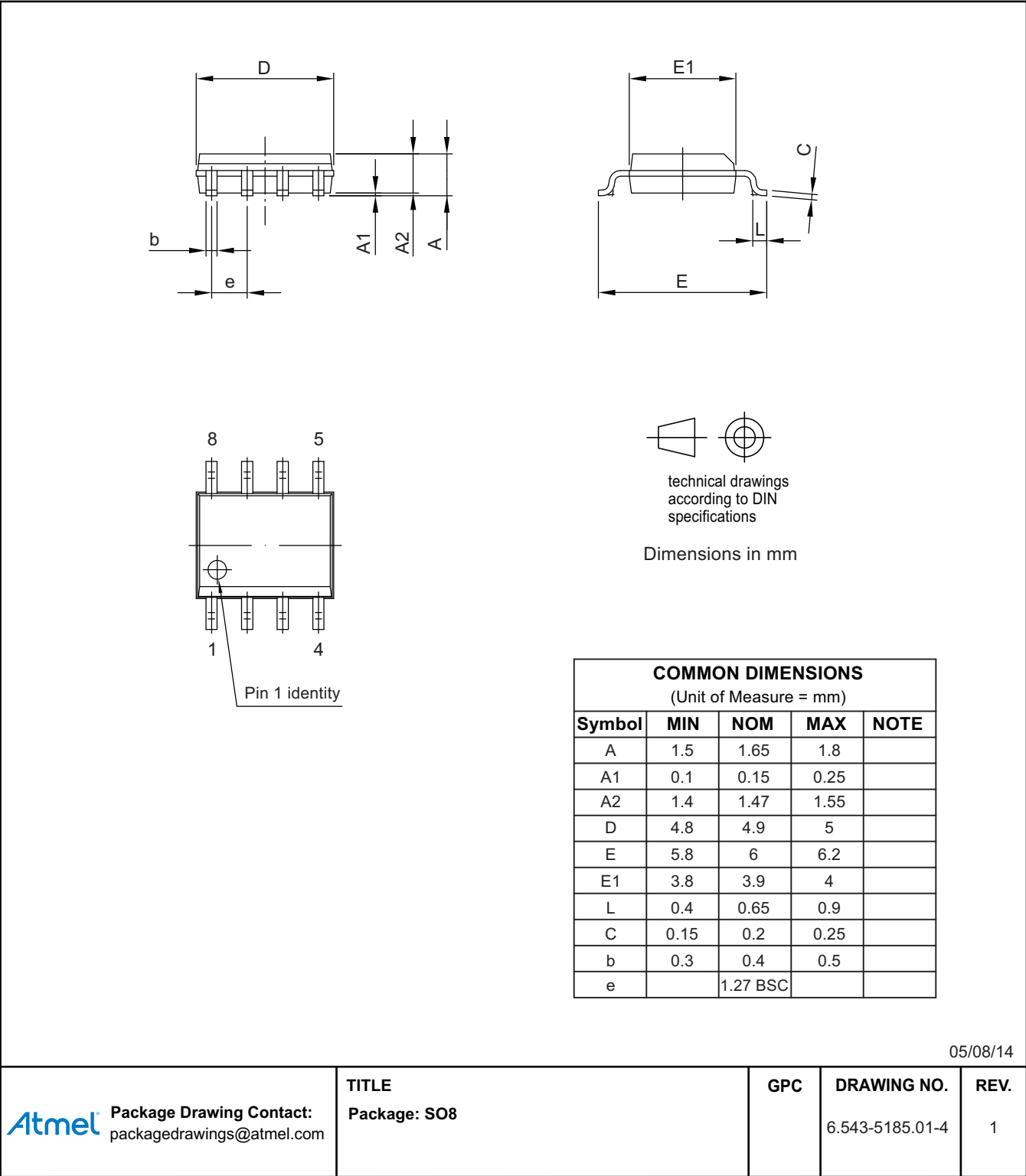
Figure 9-1. SO8
