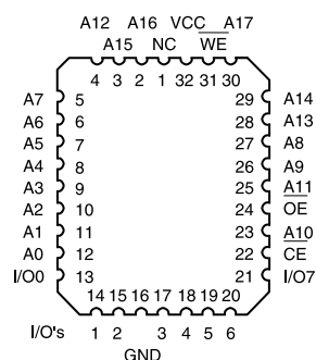
PLCC Top View
