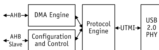
Figure 2-16. USB Interface
