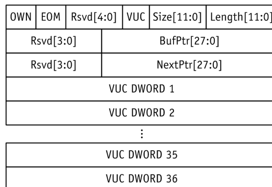
Figure 4-3. DMA Descriptor Structure
