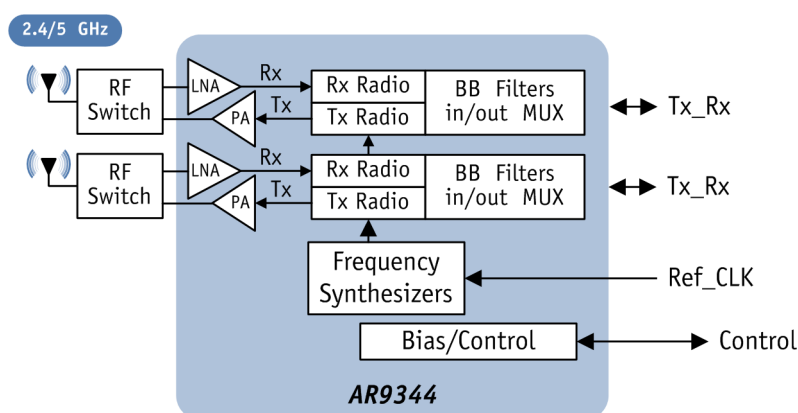
Figure 7-1. Radio Functional Block Diagram
