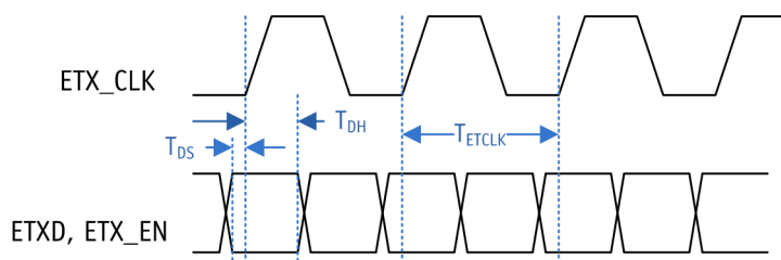
Figure 10-5. MII Mode Timing
