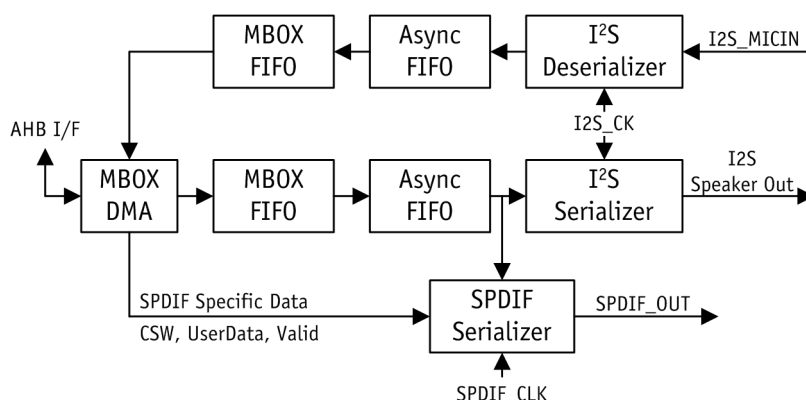
Figure 4-1. Audio Interface
