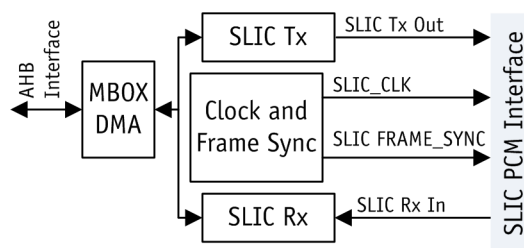
Figure 2-8. SLIC Block Diagram
