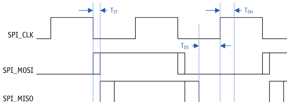
Figure 10-6. SPI Timing
