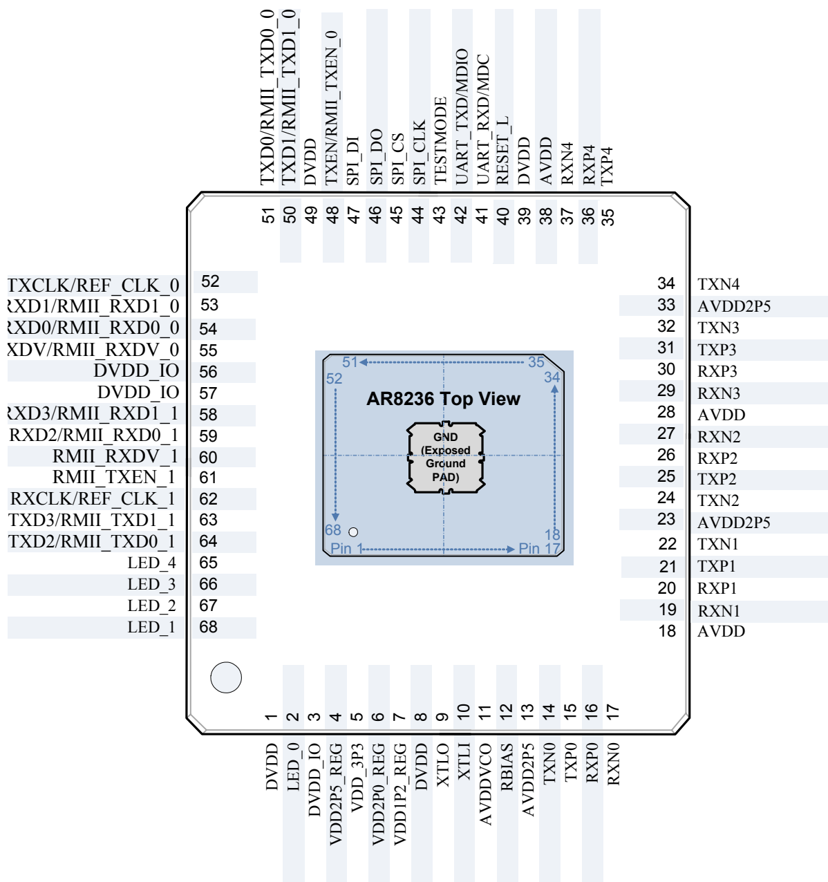
Figure 1-1. 68 pin QFN Package Pinout
