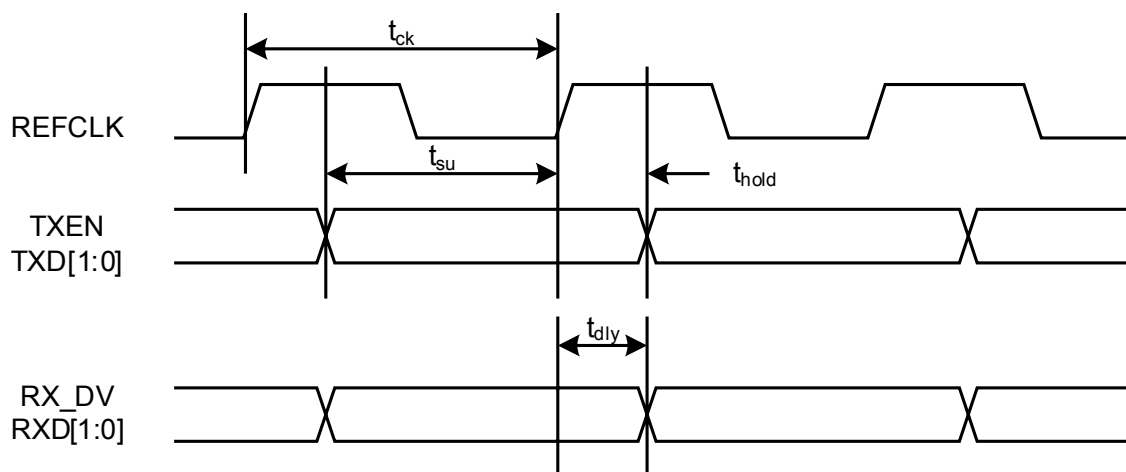
Figure 5-4. RMII Input Timing Diagram
