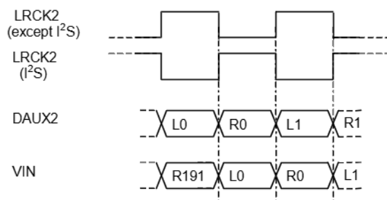
Figure 22. DAUX2 and VIN input timings
