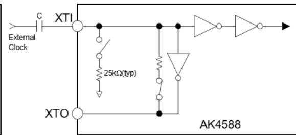
Figure 19 (3.3V). (b). External clock
