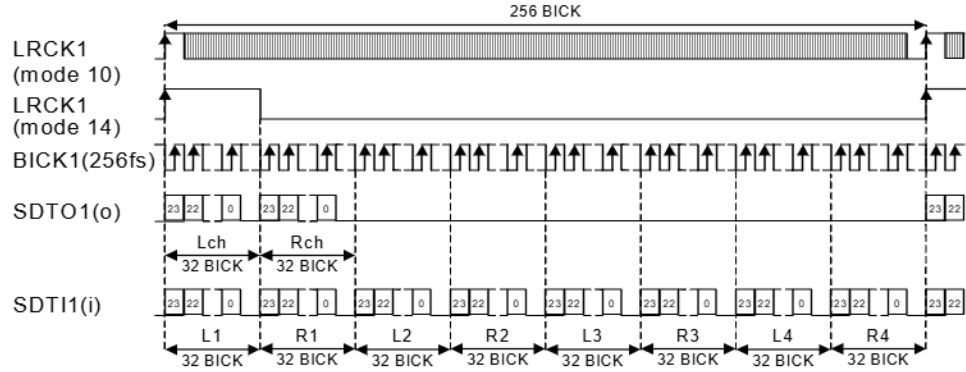
Figure 7. Mode 10 ,14 Timinig
