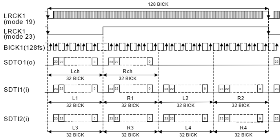
Figure 12. Mode 19 ,23 Timing
