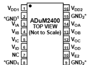
Figure 5. ADuM2400 Pin Configuration
