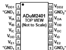
Figure 6. ADuM2401 Pin Configuration
