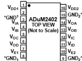
Figure 7. ADuM2402 Pin Configuration
