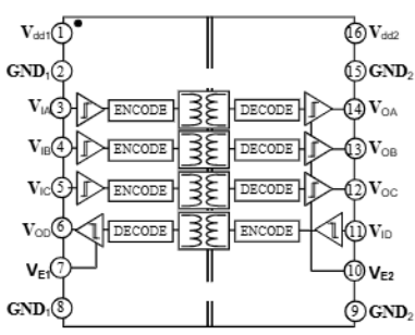
Figure 2. ADuM2401 Functional Block Diagram
