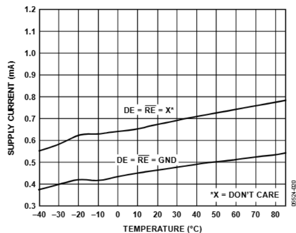
Figure 30. Supply Current vs. Temperature
