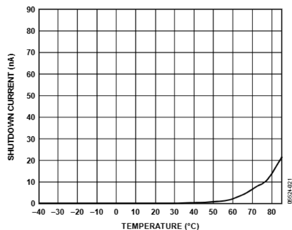
Figure 31. Shutdown Current vs. Temperature
