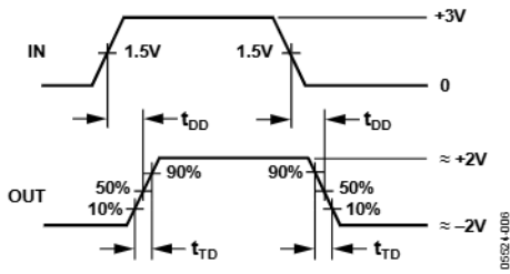
Figure 16. Driver Differential Output Delay and Transition Times
