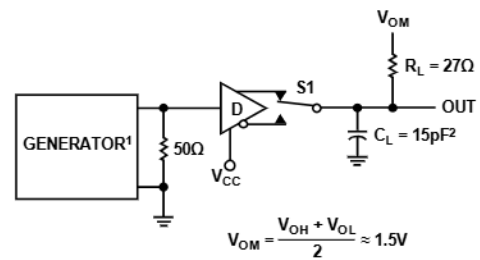
Figure 10. Driver Differential Output Delay and Transition Times
