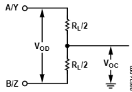
Figure 7. Differential Output Voltage and Common-Mode Voltage Drivers
