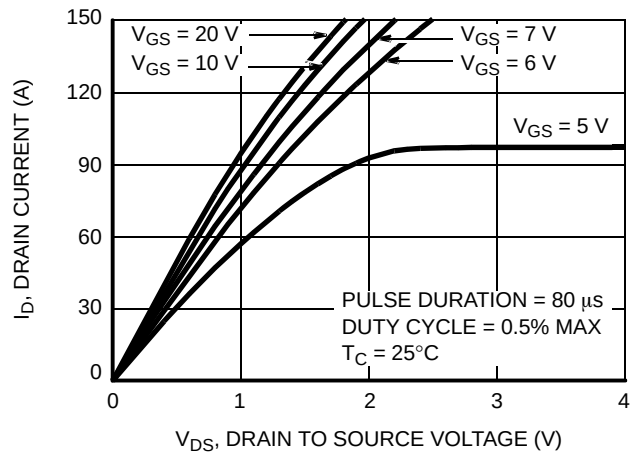
Figure 8. Saturation Characteristics
